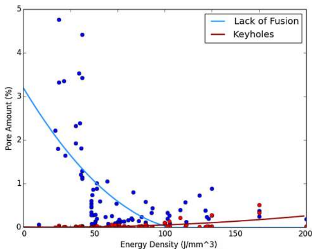
Fig. 4. Percentage of pores classified plotted against the energy density of the data set. The pore percentages were calculated using limits 70\ \mu\text{m} for the pore length and 0.7 for the roundness for both types of pore.
