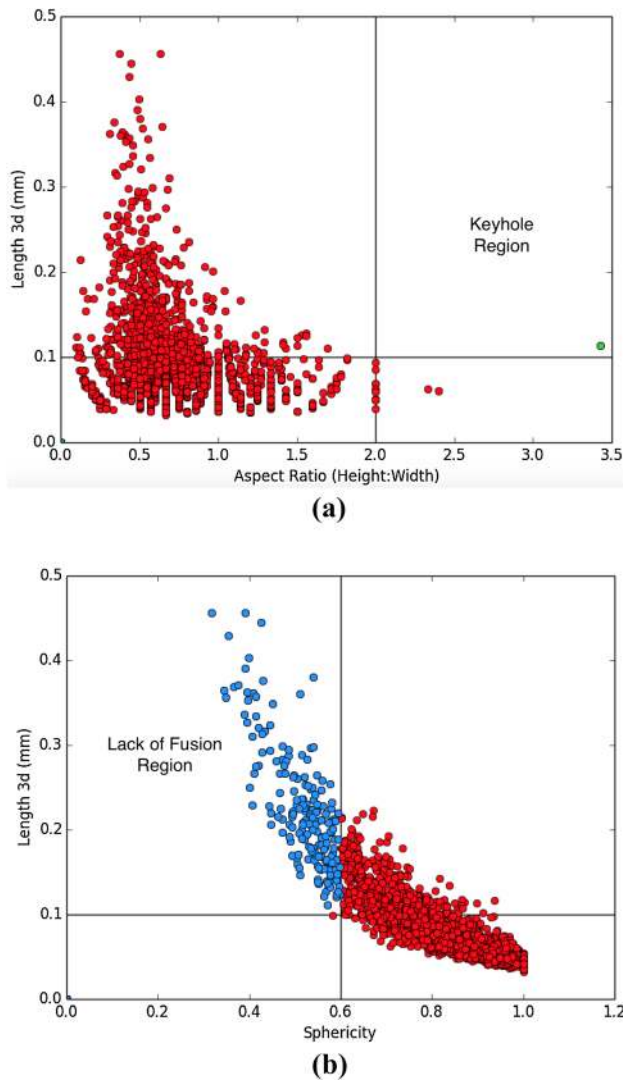
Fig. 5. The 3D pore sample data. All non-classified pores are shown in red. (a) The length and aspect ratio (in the build direction) of the pores. The KH region is labelled with the KH pore shown in green. (b) The length and sphericity of the pores. The LF region is labelled with the LF pores shown in blue (Color figure online).
