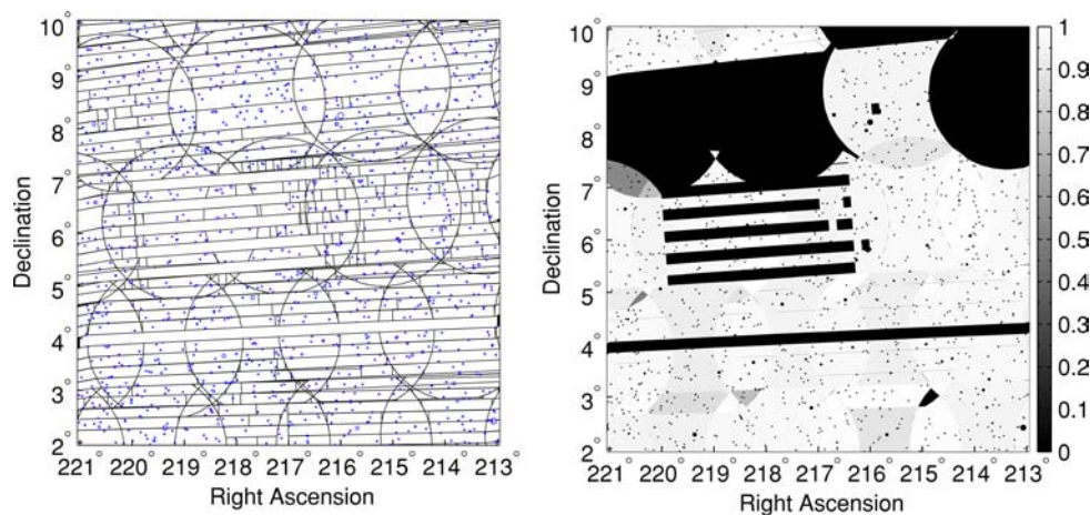
Figure 2. A portion of the SDSS DR5 angular mask (Blanton et al. 2005; Adelman-McCarthy et al. 2007). Left-hand panel: Polygons defining the mask: spectroscopic plates and lines delineating different scans and spectroscopic plates are shown in black, and holes in the mask are shown in blue/grey. Right-hand panel: Processed version of the mask, shaded according to survey completeness.
