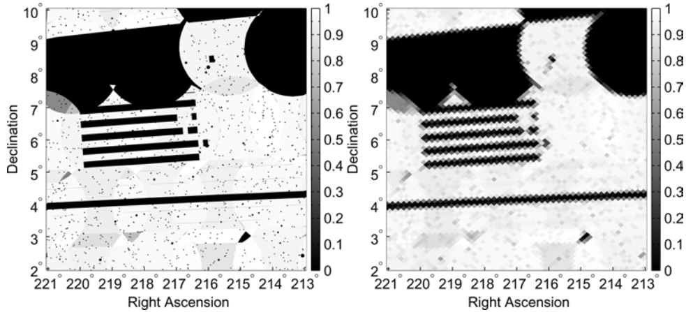
Figure 8. Left-hand panel: portion of SDSS mask as shown in Fig. 2. Right-hand panel: portion of SDSS mask from Fig. 2 as approximated by HEALPIX pixels, rasterized to N_{\text{side}} = 512 .
