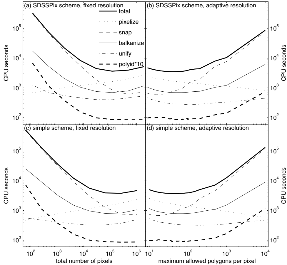
Figure 7. Time required to process the full SDSS DR5 mask with different choices of pixelization schemes and methods. The ‘total’ curves are the sum of the pixelization, snapping, balkanization and unification curves. Also shown is the time required to identify in which polygon each of the \sim 400\,000 SDSS DR5 galaxies lies (polyid), scaled up by a factor of 10. The plots on the left-hand side show time versus the number of pixels at a fixed resolution. The plots on the right-hand side show time versus N_{\max} , the maximum number of polygons in allowed in each pixel when pixelizing with the adaptive resolution method.
