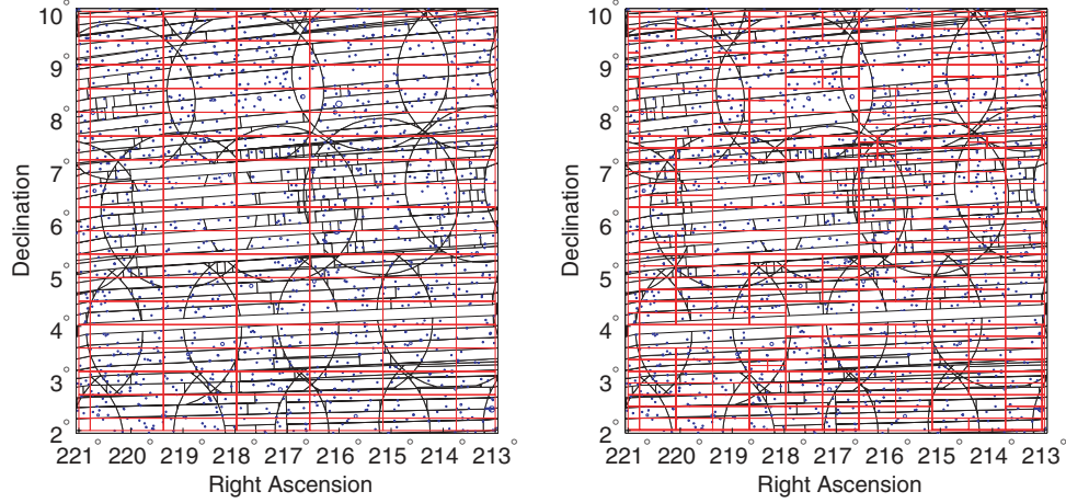
Figure 6. Left-hand panel: portion of SDSS mask from Fig. 2 pixelized to resolution 8 ( 4^8 total pixels on the sky) with the simple pixelization scheme. Pixel boundaries are shown in red/light grey. Right-hand panel: the same mask pixelized with the simple pixelization scheme using the adaptive resolution method with a maximum of 30 polygons per pixel.
