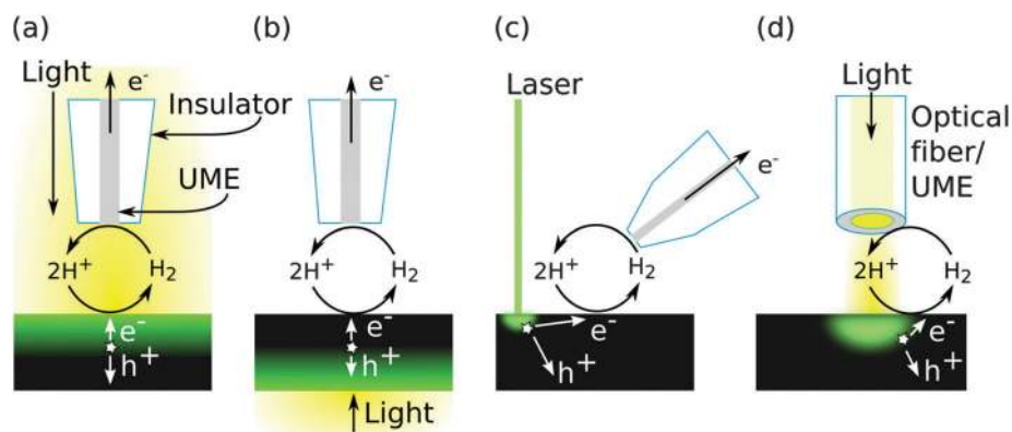
Fig. 2 Schematic side-views of several SECM set-up arrangements that can be used for investigating photoelectrode surfaces. Schematics not to scale. Schematics illustrate \text{H}_2 evolving from a photocathode surface, but identical illustrations could be drawn for photoanodes evolving \text{O}_2 . The light green regions in the figure represent the photon absorption/charge carrier generation volume in the semiconducting photoelectrode.
