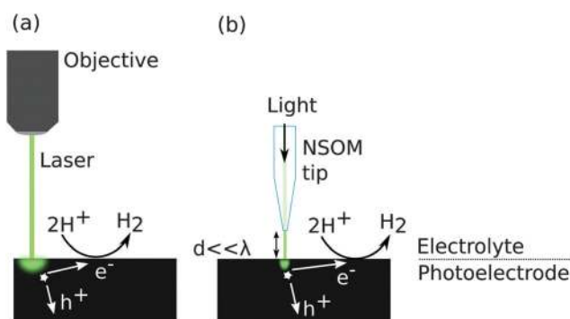
Fig. 1 Schematics of (a) conventional and (b) NSOM-based SPCM set-ups for in situ scanning photocurrent analysis of photoelectrodes for water splitting. Schematics not to scale. Schematics illustrate \text{H}_2 evolving from a photocathode surface, but identical illustrations could be drawn for photoanodes evolving \text{O}_2 . The light green regions in the figure represent the photon absorption/charge carrier generation volume in the semiconducting photoelectrode.
