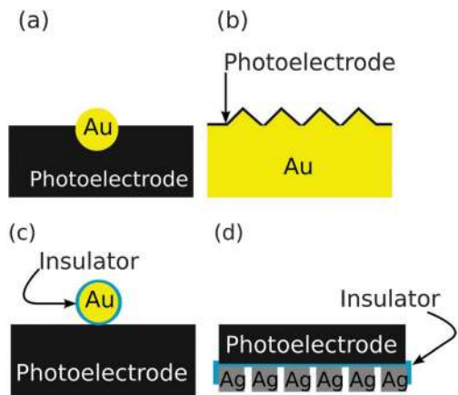
Fig. 3 Strategies for generating localized surface plasmon resonance on photoelectrode surfaces that could be used for SERS characterization: (a) Au nanoparticles embedded in a photoelectrode (after ref. 135); (b) photoelectrode material deposited over Au nanopillars in an “overlay SERS” configuration (after ref. 136); (c) ultra-thin \text{SiO}_2 or \text{Al}_2\text{O}_3 coated Au nanoparticles deposited over a photoelectrode (after ref. 144); (d) PEC material deposited over Ag nanocubes coated with ultra-thin \text{Al}_2\text{O}_3 insulator (after ref. 143).
