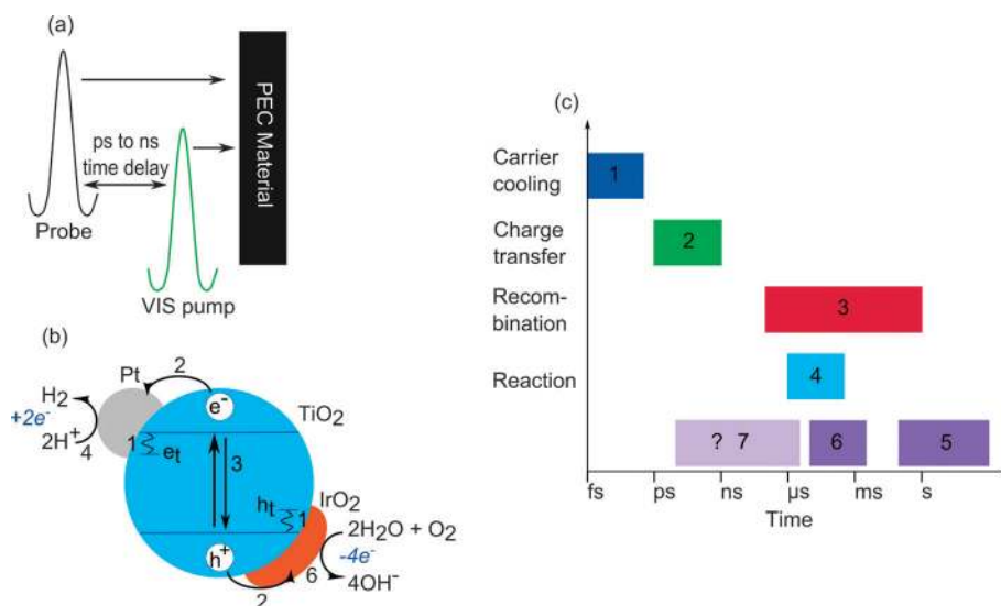
Fig. 4 (a) Schematic of a generic ultrafast pump-probe spectroscopy experiment. (b) Photophysical processes and (c) their approximate time scales for different steps in PEC water splitting for an example system comprising TiO 2 nanoparticles decorated with Pt and IrO 2 catalytic nanoparticles. Steps include instantaneous photo excitation, (1) carrier cooling and trapping, (2) interphase electron transfer from TiO 2 to Pt, (3) geminate recombination, (4) hydrogen evolution reaction on Pt catalyst, (5) O 2 evolution on TiO 2 , (6) O 2 evolution on Pt or IrO 2 , and (7) prospective O 2 evolution for next-generation OER catalysts.
