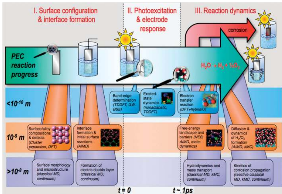
Fig. 5 Schematic of various processes and stages contributing to the complete PEC water splitting reaction (green arrow), along with possible computational methods for treating the associated physical or chemical phenomena at different length and time scales. The vertical position on the graph corresponds to the relative length scale of the process, whereas the position of the wedge where it intersects with the green arrow indicates its relative time scale.
