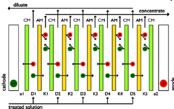
Fig. 1 Electrodialysis principles (Chen, 2004) CM – cation exchange membrane, D-diluate chamber, e1 and e2-electrode chambers, AM-anion exchange membrane and K-concentrate chamber
