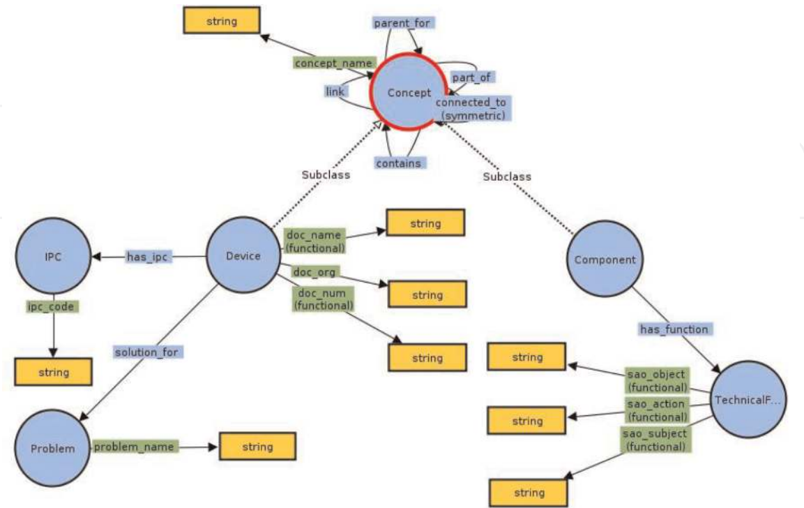
Figure 11. Ontology scheme for storing patent information.
