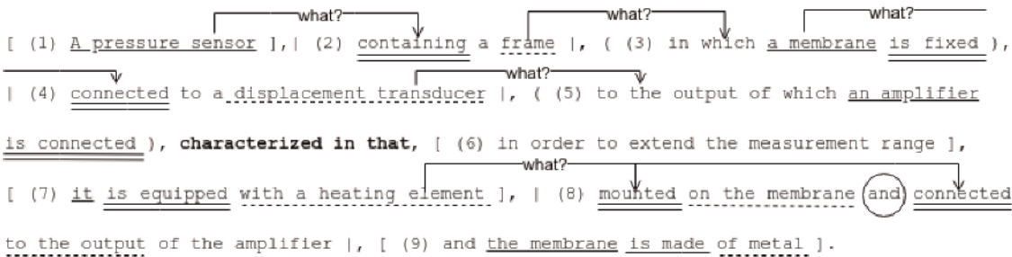
Figure 2. Parsing sentence.
