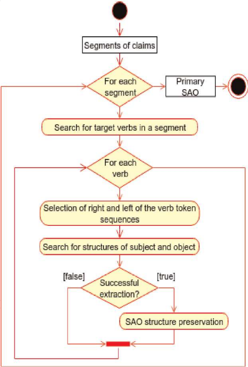
Figure 6. The general algorithm for extracting SAO structures.
