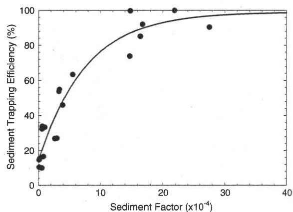
Fig. 1 Comparison of sediment factor values and corresponding values for sediment trapping efficiency (percent of input load deposited in the buffer) (Dosskey et al. 2006) estimated using VFSMOD (Muñoz-Carpena and Parsons 2000). The fitted curve is given by Eq. 2
