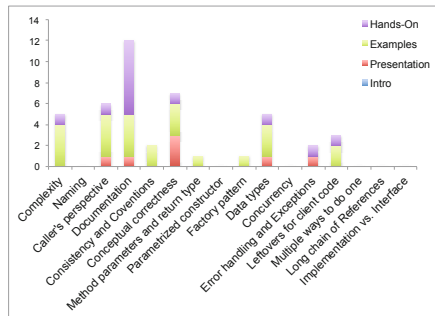
(b) API relevant usability findings
