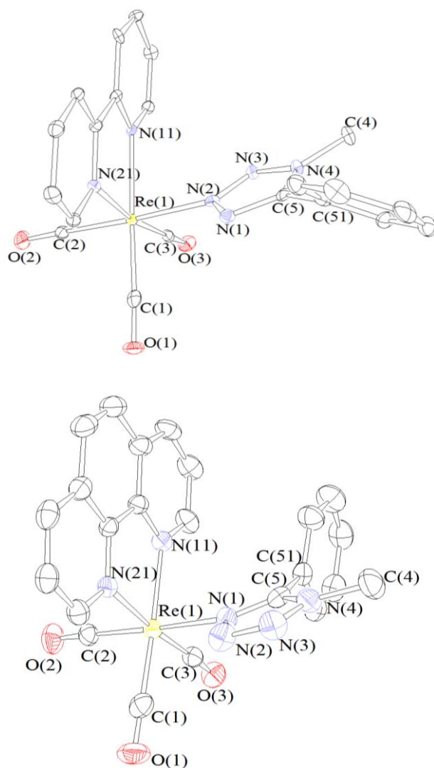
Figure 2. X-ray crystal structures of the N2 linkage isomer of fac -[Re( bipy )(CO) 3 ( TphCH 3 )] + (top) and the N1 linkage isomer of fac -[Re( phen )(CO) 3 ( TphCH 3 )] + (bottom) with key atoms labelled. Displacement ellipsoids are at 30% probability level. H-atoms and PF 6 - anions are omitted for clarity.
