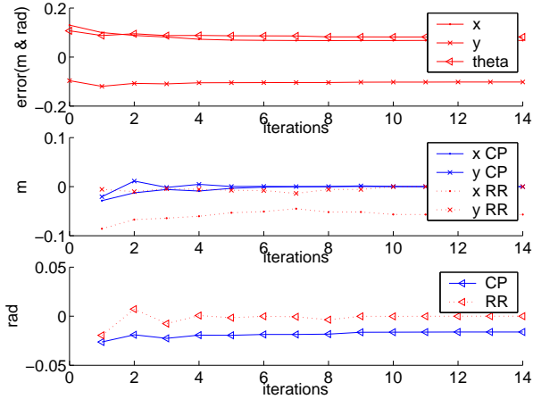
Fig. 6. The figure shows the error in location of the scan, and the corrections computed by each set of correspondences, closest point (CP) and matching range rule (RR), at each iteration of the IDC algorithm. The initial error was (0.13, -0.09, 0.1) .
