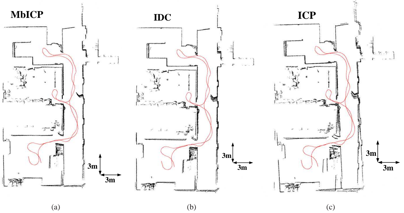
Fig. 5. (a) Visual map obtained with the MbICP. (b) Visual map of the IDC. (c) Visual map of the ICP.
