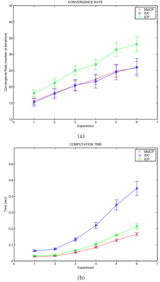
Fig. 4. (a) Mean and 0.2 times the standard deviation of the convergence rate and (b) mean and 0.2 times the standard deviation of the execution time.
