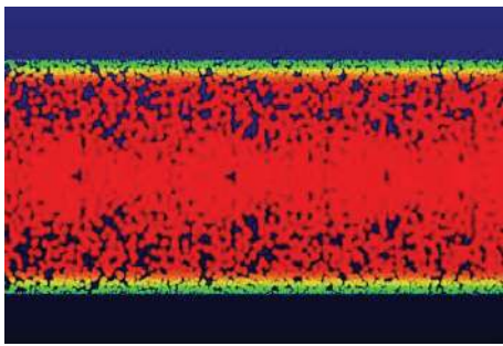
FIGURE 3: Schematic representation of particle positions based on the evaluation of the concentration of particles using the shear-induced particle migration approach.
