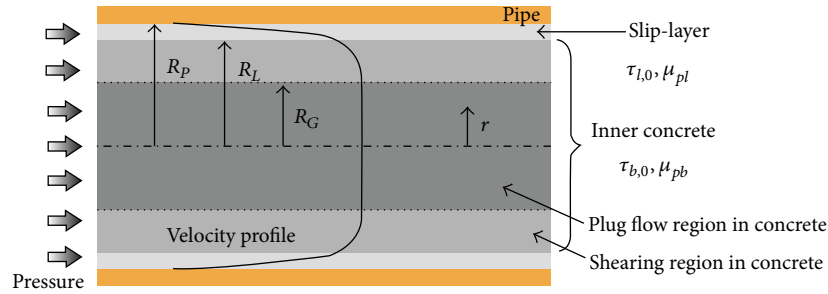
FIGURE 1: Profile of concrete flow in a pipe [4].
