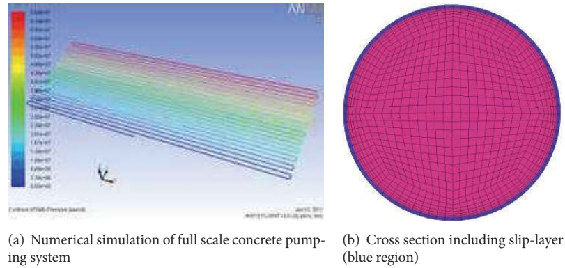
FIGURE 2: Modeling for single phase fluid approach.
