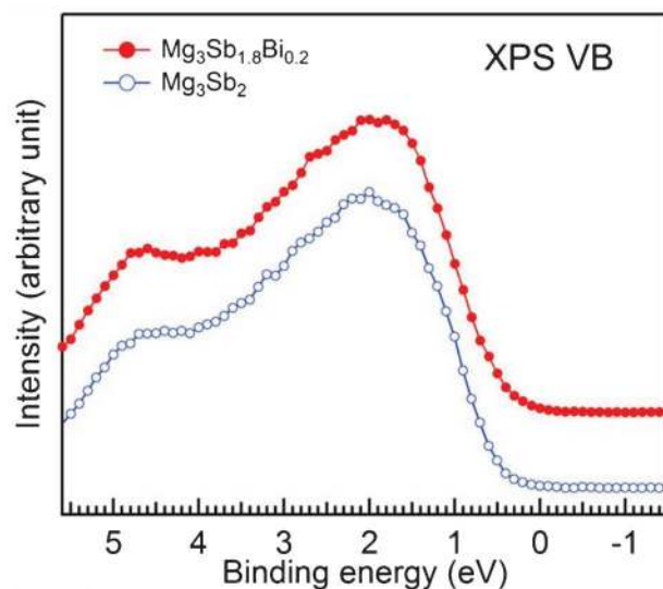
Fig. 9 XPS valence band of \text{Mg}_3\text{Sb}_2 (open circle) and \text{Mg}_3\text{Sb}_{1.8}\text{Bi}_{0.2} (filled circle). Spectra have been normalized to have the same height at their peak.
