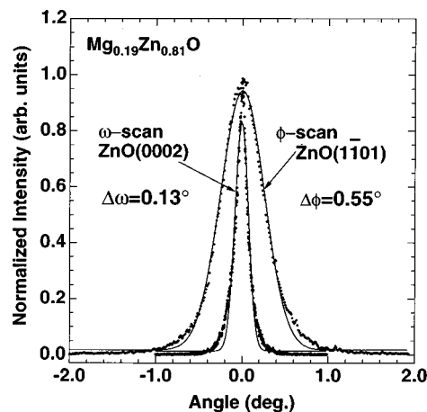
FIG. 3. X-ray diffraction rocking curves showing (0002) \omega and (1101) \phi scans of a \text{Mg}_{0.19}\text{Zn}_{0.81}\text{O} film. The width of the peaks are comparable to the highest quality pure ZnO films.
