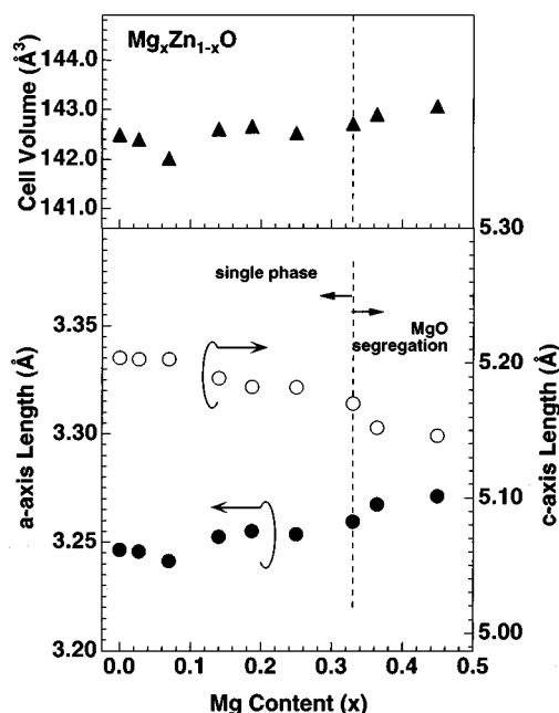
FIG. 2. Mg content dependences of the a - and c -axis lattice parameters and the cell volume of \text{Mg}_x\text{Zn}_{1-x}\text{O} films. Segregation of the MgO impurity phase was observed for x \geq 0.33 of Mg content.
