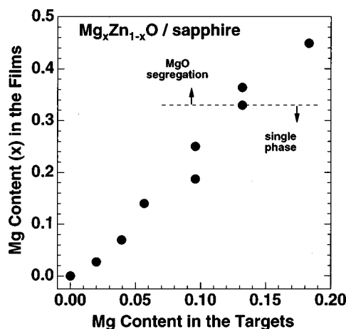
FIG. 1. Mg content in the \text{Mg}_x\text{Zn}_{1-x}\text{O} epitaxial films as a function of target Mg content.
