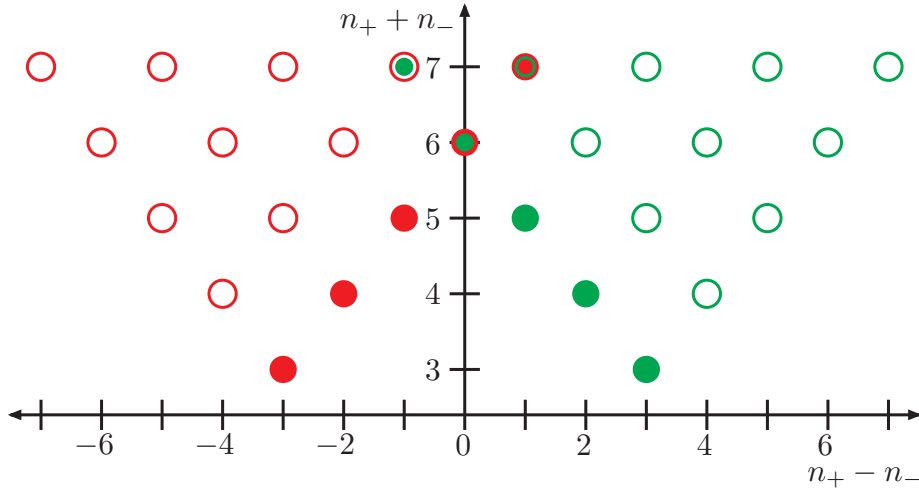
Figure 8: The proposed structure of n -gluon amplitudes induced by the operator \text{tr}(G^3) . The MHV tower for \text{tr}(G^3_{SD}) -induced amplitudes contains pure MHV vertices (closed red circles) plus those amplitudes obtained by adding pure-gauge-theory MHV vertices (open red circles). The anti-MHV tower of \text{tr}(G^3_{ASD}) -induced amplitudes is obtained from the MHV tower by parity, and is shown in green. The \text{tr}(G^3) -induced amplitudes are given by the sum of the two contributions, where they overlap. The two entries with n_+ + n_- = 3 represent MHV vertices, but not on-shell scattering amplitudes.
