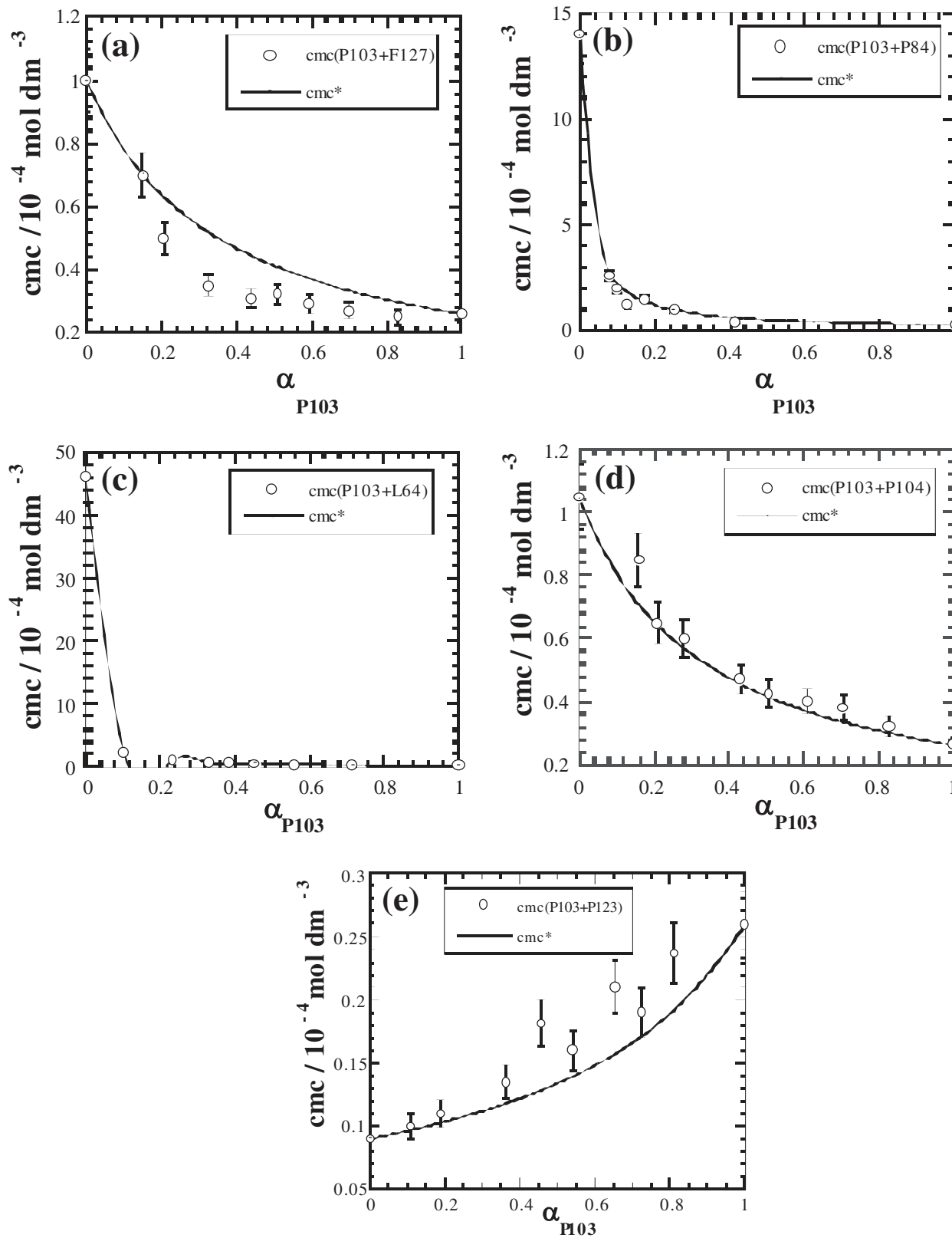
Figure 3 Critical micelle concentration versus mole fraction of P103. For (a) P103 + F127, (b) P103 + P84, (c) P103 + L64, (d) P103 + P104, and (e) P103 + P123 binary mixtures, respectively.
