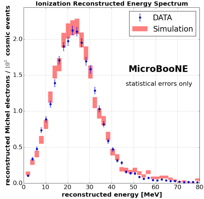
Figure 16: Reconstructed energy spectrum for the measured ionization-only Michel electron energy. The performance of the reconstruction algorithm on data and Monte Carlo events are compared. Error bars represent statistical uncertainties only for both data and simulation.
