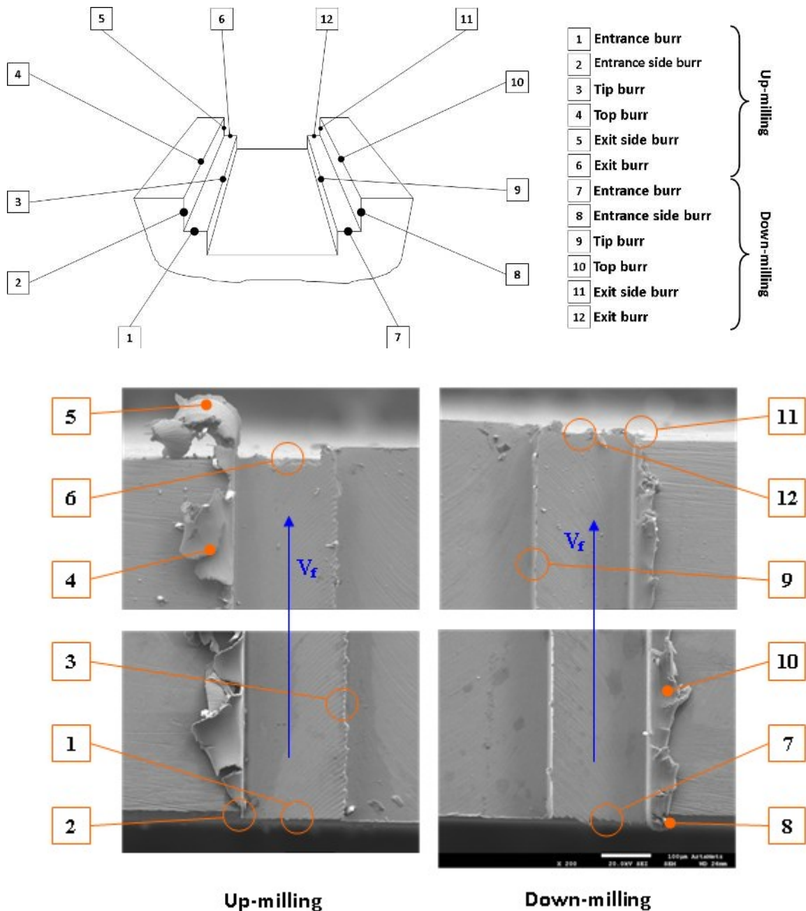
Fig. 5 : Entrance and exit of tests n°3 and n°4
