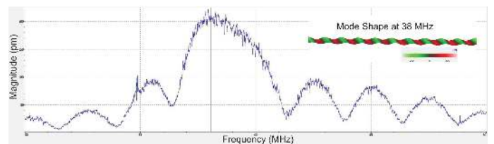
Fig. 3 The resonance mode of a SAW device is revealed by this graph of amplitude vs frequency at a single point over an averaging period while the device is driven with a multi-frequency signal. Once this resonance is known, a sequential measurement over a region of the surface while the device is driven at the resonance frequency reveals the vibration mode, SAW in this case.
