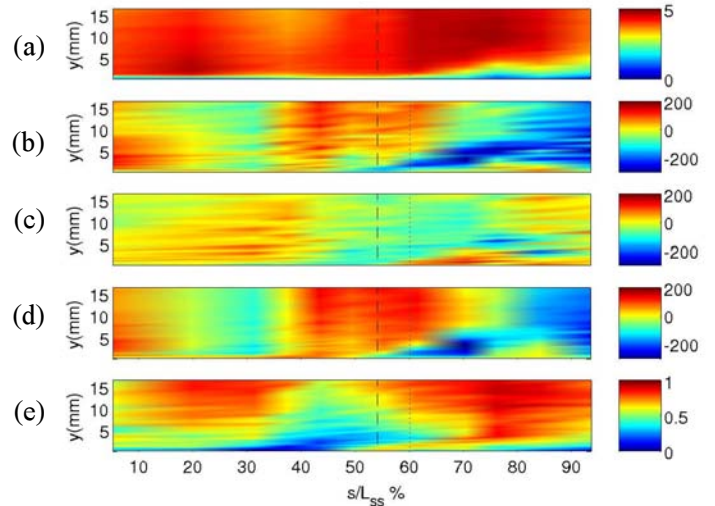
Fig. 4 One picture from one movie ((a) velocity, (b) Du/Dt , (c) \frac{\partial u}{\partial t} , (d) u\frac{\partial u}{\partial x} , (e) intermittency). This is at \theta=320^\circ . Color scale indicates values of the parameter, plotted vs. distance from wall, y (mm), and streamwise distance, s , is normalized on suction surface length, L_{ss} . The dashed line is transition onset and the dotted line is separation.
