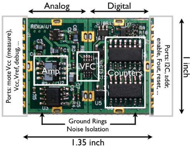
Figure 2: The scalable power observation tool (SPOT) consists of a sense resistor, amplifier, voltage-to-frequency converter, and two counters.
