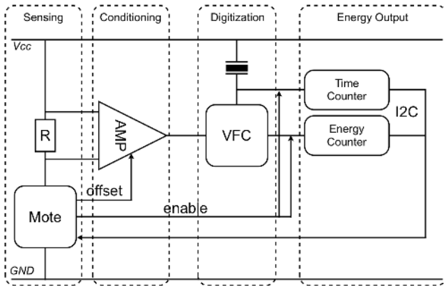
Figure 5: Architecture and Primary Components
