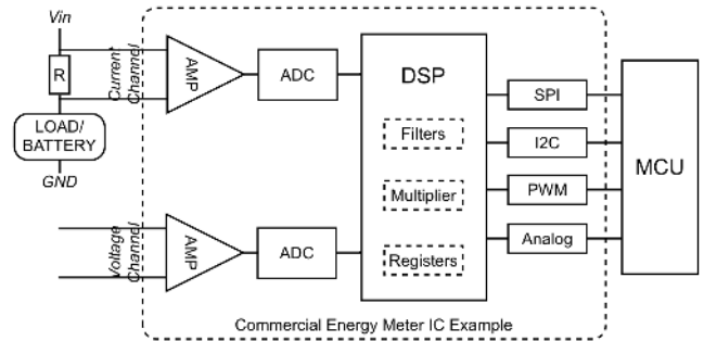
Figure 4: Architecture of a typical energy metering circuit.
