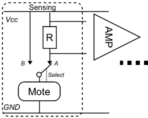
Figure 6: SPDT Switch for Calibration. In one configuration, current flow bypasses the shunt resistor, allowing the input offset to be measured. In the other configuration, current passes through the shunt resistor, allowing the mote current to be measured.
