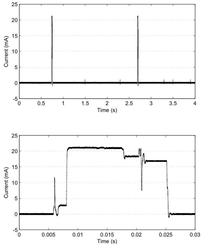
Figure 1: A typical nodal current profile consists of long periods of low-current sleep punctuated by short, periodic bursts of high-current activity.
