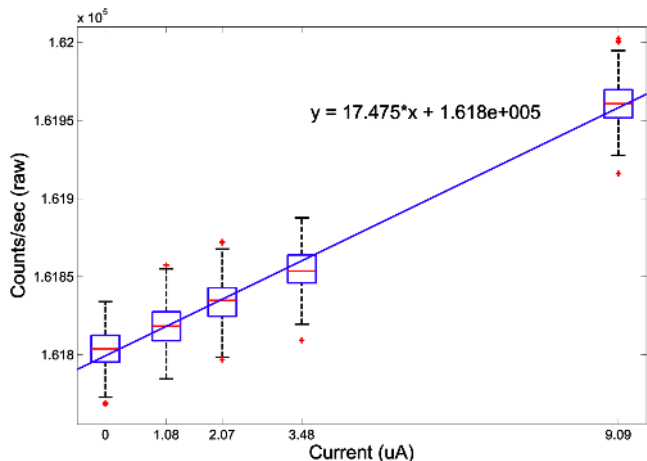
Figure 12: SPOT current resolution. SPOT can resolve currents at the microamp level.
