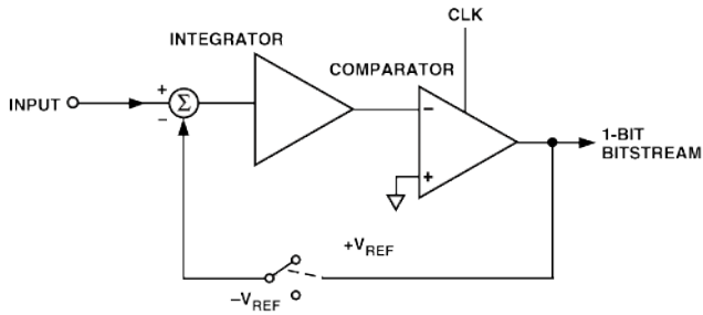
Figure 9: The architecture of a VFC.
