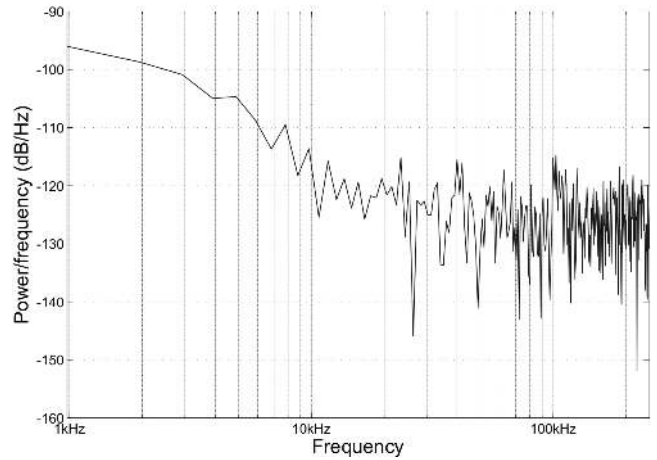
Figure 3: The power spectral density of a node current profile shown in Figure 1.
