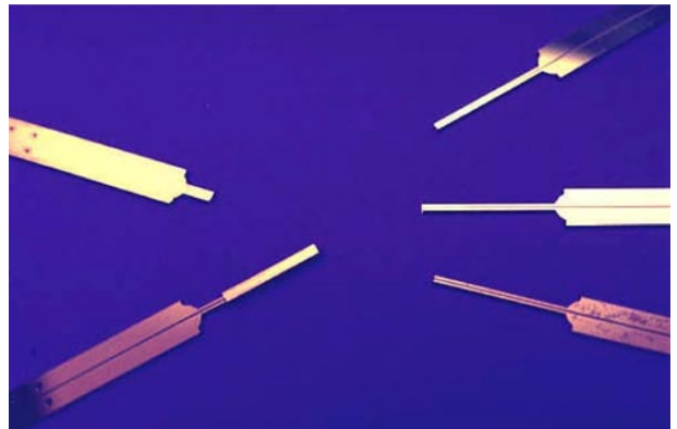
Figure 6. Micromachined ultrasonic needles (from [14]).
