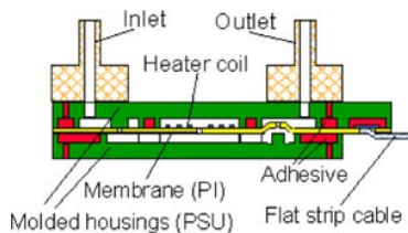
Figure 4. Schematic diagram of a micropump (from [13]).
