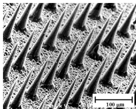
Figure 10. Micromachined needles for transdermal drug release (from [21]).
