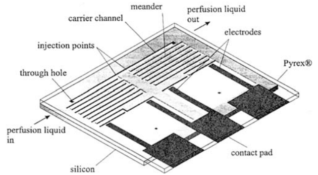
Figure 2. Schematic diagram of two micromachined pumps and dosing systems (from [11]).
