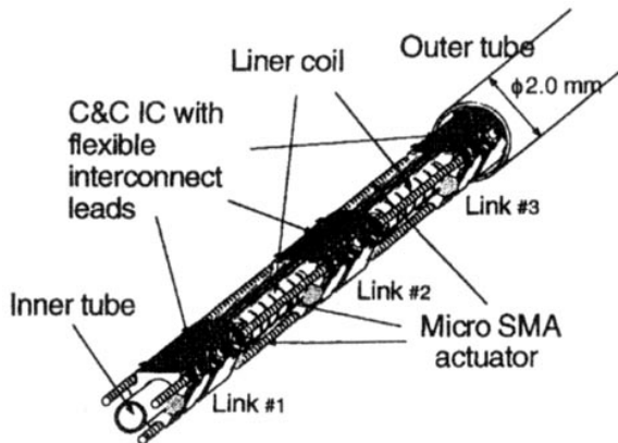
Figure 19. Active microcatheter with integrated circuits (from [39]).
