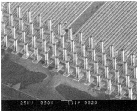
Figure 16. Array of microneedles for selective nerve stimulation (from [33]).
