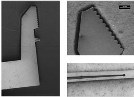
Figure 22. SEM micrographs of a nickel microgripper (from [43]).
