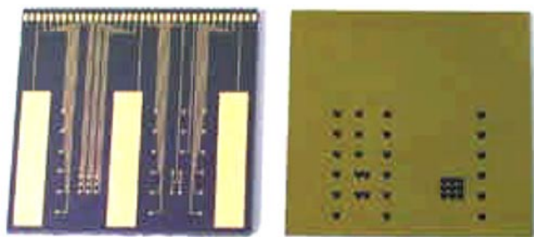
Figure 12. Front (left) and back (right) views of the controlled release microchip (from [25]).
