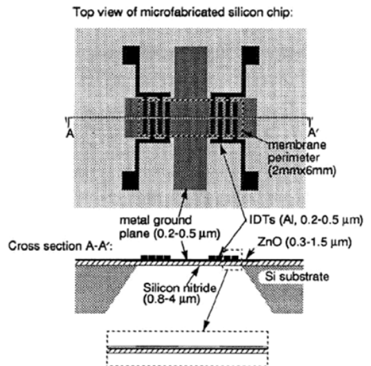
Figure 5. Schematic diagrams of an ultrasonic flexural plate wave device (from [14]).
