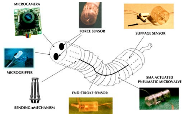
Figure 21. Concept of minirobot for MIT and MIS, with existing miniature components.
