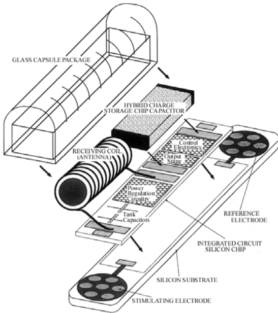
Figure 15. Single-channel, implantable microstimulator (from [32]).
