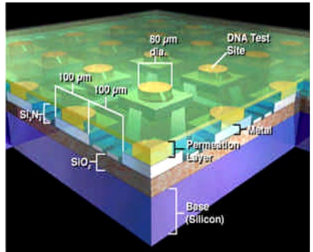
Figure 9. A view of the microchip structure (from [20]) developed by Nanogen Inc., San Diego, California, USA.
