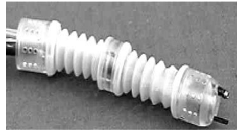
Figure 20. Mini-robot for colonoscopy.
