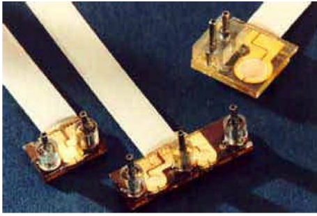
Figure 3. Examples of micropump prototypes developed at Karlsruhe University (from [13]).
