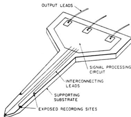
Figure 14. Silicon probe for neural recording (from [29]).
