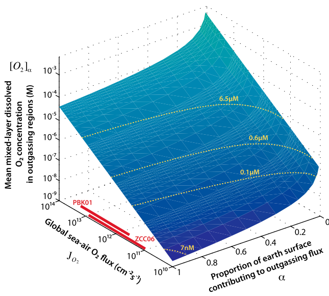
Fig. 4. The modeled average dissolved oxygen concentration in oxygenated regions of the Archean surface ocean, as a function of the sea-to-air O_2 flux and the proportion of the Earth's surface contributing to that flux. The larger the outgassing flux, and the smaller the fraction of the earth's surface it comes from, the more oxygenated surface waters in that region must be. Yellow contours indicate the dissolved oxygen concentrations of the steroid biosynthesis experiments (7 nM, 0.6 \mu M, and 6.5 \mu M) and the detection limit of the oxygen microelectrode (0.1 \mu M). Red bars indicate the range of O_2 fluxes in the Archean atmospheric evolution models of Pavlov et al. (21) (PBK01) and Zahnle et al. (22) (ZCC06).
