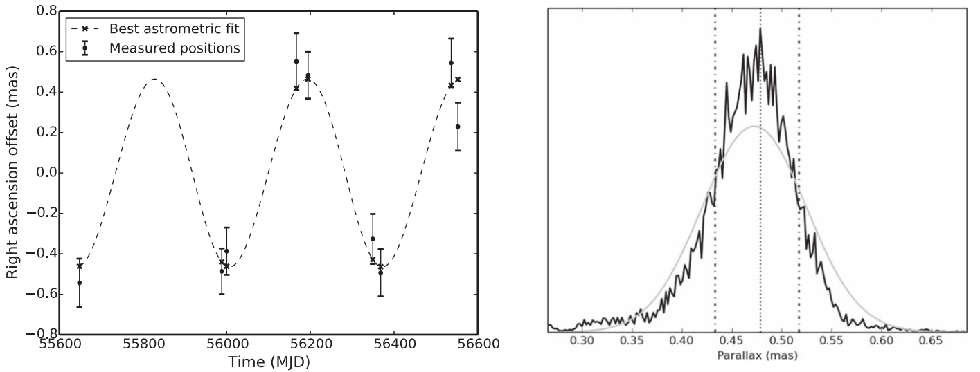
Figure 8. Effect of including an empirical estimate of the systematic error based on the calibrator-target separation and calibrator flux density. Left: least-squares fit to data set with systematic error estimates included: offset in R.A. is shown as a function of time, after subtracting the best-fit proper motion. The reduced \chi^2 is 1.4. Right: the bootstrap fit results for parallax, from the data set with systematic error estimates. The parallax obtained is 0.48 \pm 0.04 \mu\text{as} .
