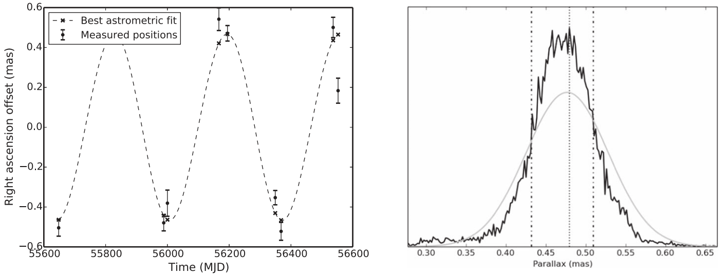
Figure 7. Effect of including an estimate of the systematic error based on the scatter between ionospheric models for PSR J0601–0527. Left: least-squares fit to data set with systematic error estimates included: offset in R.A. is shown as a function of time, after subtracting the best-fit proper motion. The reduced \chi^2 is 8. Right: the bootstrap fit results for parallax, from the data set with systematic error estimates. The parallax obtained is 0.47 \pm 0.04 \mu\text{as} .
