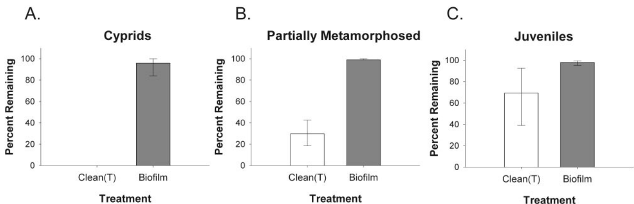
Figure 4. Mean percentage of Balanus amphitrite remaining on slides after exposure of a nominal wall-shear stress of 120 Pa. Metamorphosed individuals were evaluated at the (A) attached cyprid, (B) partially metamorphosed, and (C) post-metamorphic juvenile stages. Treatments consisted of glass slides cleaned with Triton X-100 (T) and biofilmed slides. Error bars = 1 SE.
