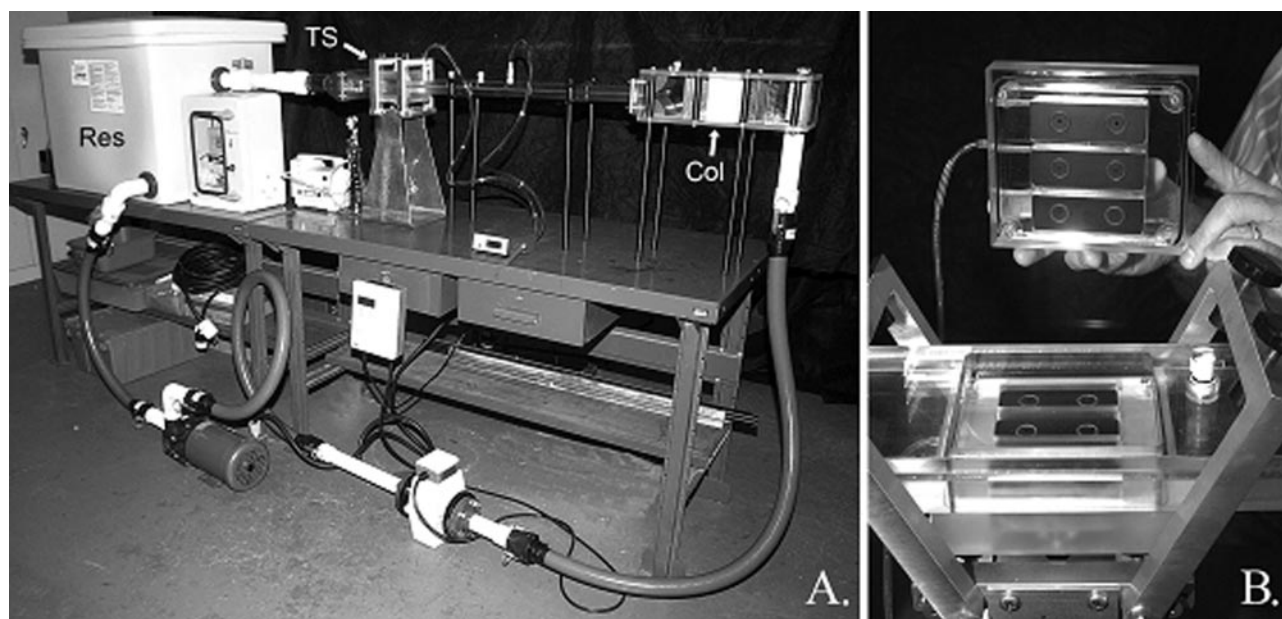
Figure 1. (A) Turbulent channel flow apparatus used in testing adhesion of four invertebrate species to glass microscope slides. Slides are held in the test chamber by a suction device. Charged with seawater, the device circulates water through a collimator (Col), the test chamber (TS), and into a receiving reservoir (Res) (for details of hydrodynamic flow see Schultz et al. , 2000). (B) Close-up of the test chamber. Photographs by Dr. M. P. Schultz, U.S. Naval Academy.
