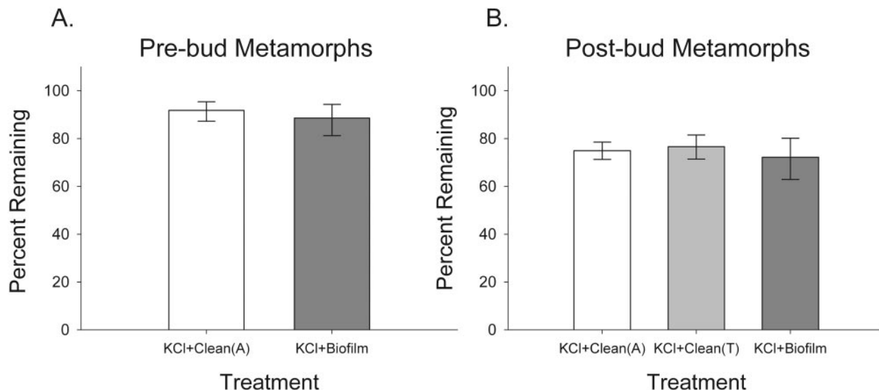
Figure 5. (A) Mean percentage of Bugula neritina at the pre-budding stage remaining on slides after exposure to 75 Pa nominal wall-shear stress. Treatments consisted of glass slides cleaned with acid (A) or biofilmed slides. (B) Mean percentage of B. neritina at the post-budding stage remaining on slides following exposure to 75 Pa nominal wall-shear stress. Treatments consisted of glass slides cleaned with acid (A), Triton X-100 (T), or coated with a natural biofilm. Excess KCl ( 10 \text{ mmol l}^{-1} ) was applied to all treatments. Error bars = 1 SE.
