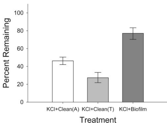
Figure 2. Mean percentage of Phallusia nigra remaining on slides after exposure to a nominal wall-shear stress of 120 Pa. Treatments consisted of glass slides cleaned with acid (A) or Triton X-100 (T), or coated with a natural biofilm. Excess KCl ( 10 \text{ mmol l}^{-1} ) was applied to all treatments. Error bars = 1 SE.
