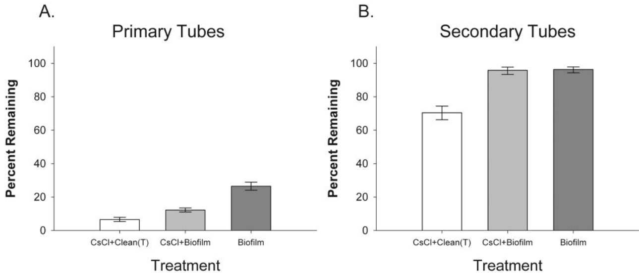
Figure 3. Mean percentage of Hydroides elegans remaining on slides after exposure to a nominal wall-shear stress of 50 Pa. Metamorphosed individuals of H. elegans were evaluated at the (A) primary and (B) secondary tube stages. The proteinaceous primary tube is secreted shortly after the initiation of metamorphosis. The secondary tube is calcified and secreted after metamorphosis. Treatments consisted of glass slides cleaned with Triton X-100 (T) and biofilmed slides. Excess CsCl ( 10 \text{ mmol l}^{-1} ) was used to induce larvae to metamorphose on clean slides, and as a control, larvae were exposed to biofilm and CsCl. Error bars = 1 SE.
