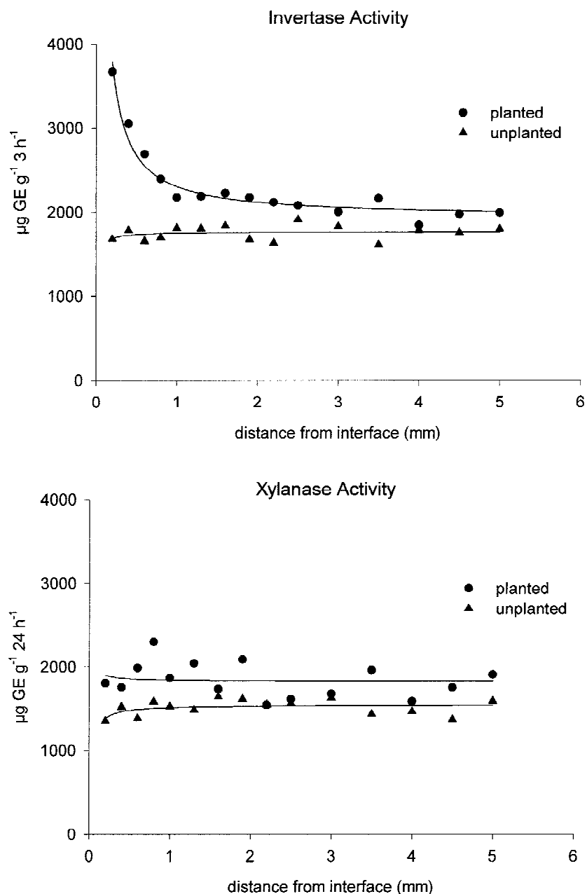
Figure 4. Small-scale variability of xylanase and invertase activities in the rhizosphere of maize and in the unplanted controls.
