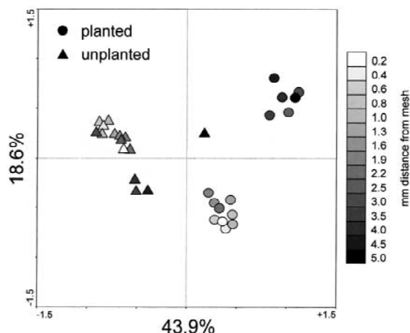
Figure 3. Ordination plot generated by principal component analysis of 16S rDNA-DGGE patterns in the rhizosphere of maize and in unplanted control. Distances from the root surface in mm.
