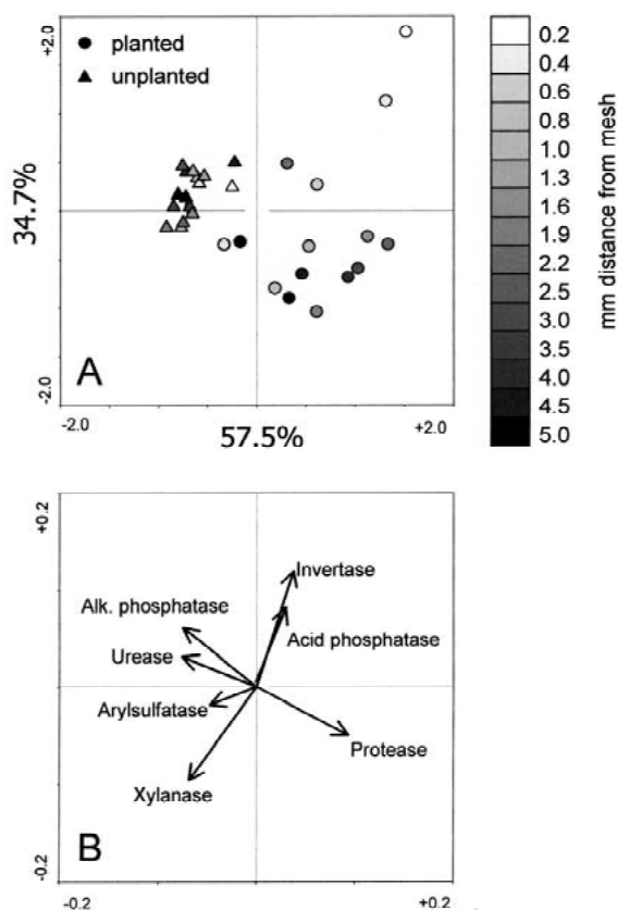
Figure 6. Ordination plot of principal component analysis of enzyme activities of samples (A) and enzymes (B) in the rhizosphere of maize and in implanted controls. Distances from the root surface in mm.
