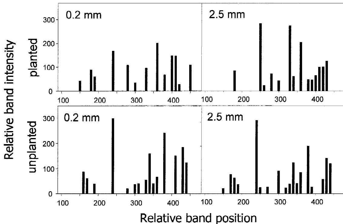
Figure 2. Digitized DGGE 16S rDNA band pattern in 0.2 and 2.5 distance from the root-soil interface and from the soil surface of the unplanted control.
