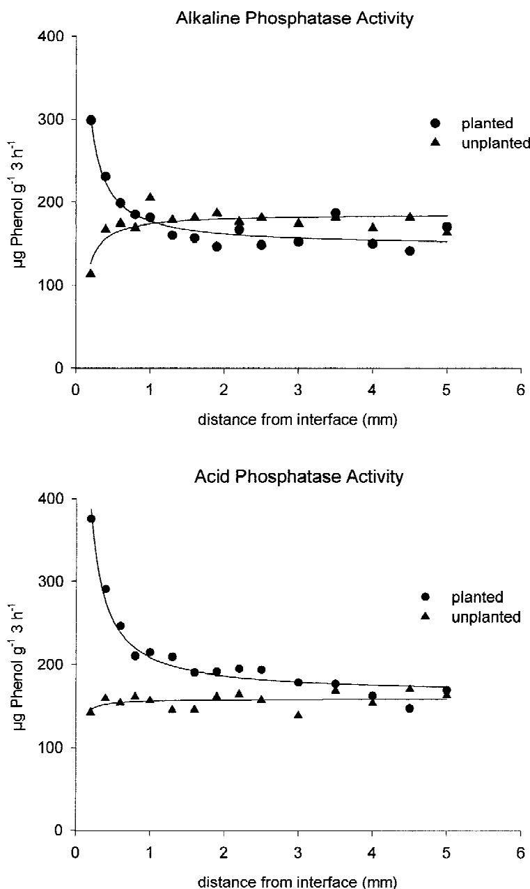
Figure 5. Small-scale variability of alkaline and acid phosphatase activities in the rhizosphere of maize and in the unplanted controls.
