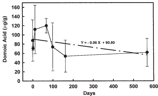
Fig. 3. Domoic acid levels ± SD in unfed sea scallops plus the regression line calculated using these values. Sixty scallops (10–12 cm diameter) collected April 28, 1988 from the Bay of Fundy were placed on the floor of a 90 × 90 cm square tank with aerated filtered flowing sea water (flow rate of 2 L/min) at ambient temperature. On day 0, eight scallops were taken to establish baseline values; all subsequent samples consisted of five scallops each selected at random. Temperatures ranged from ca. 1 to 15°C over the storage period.
