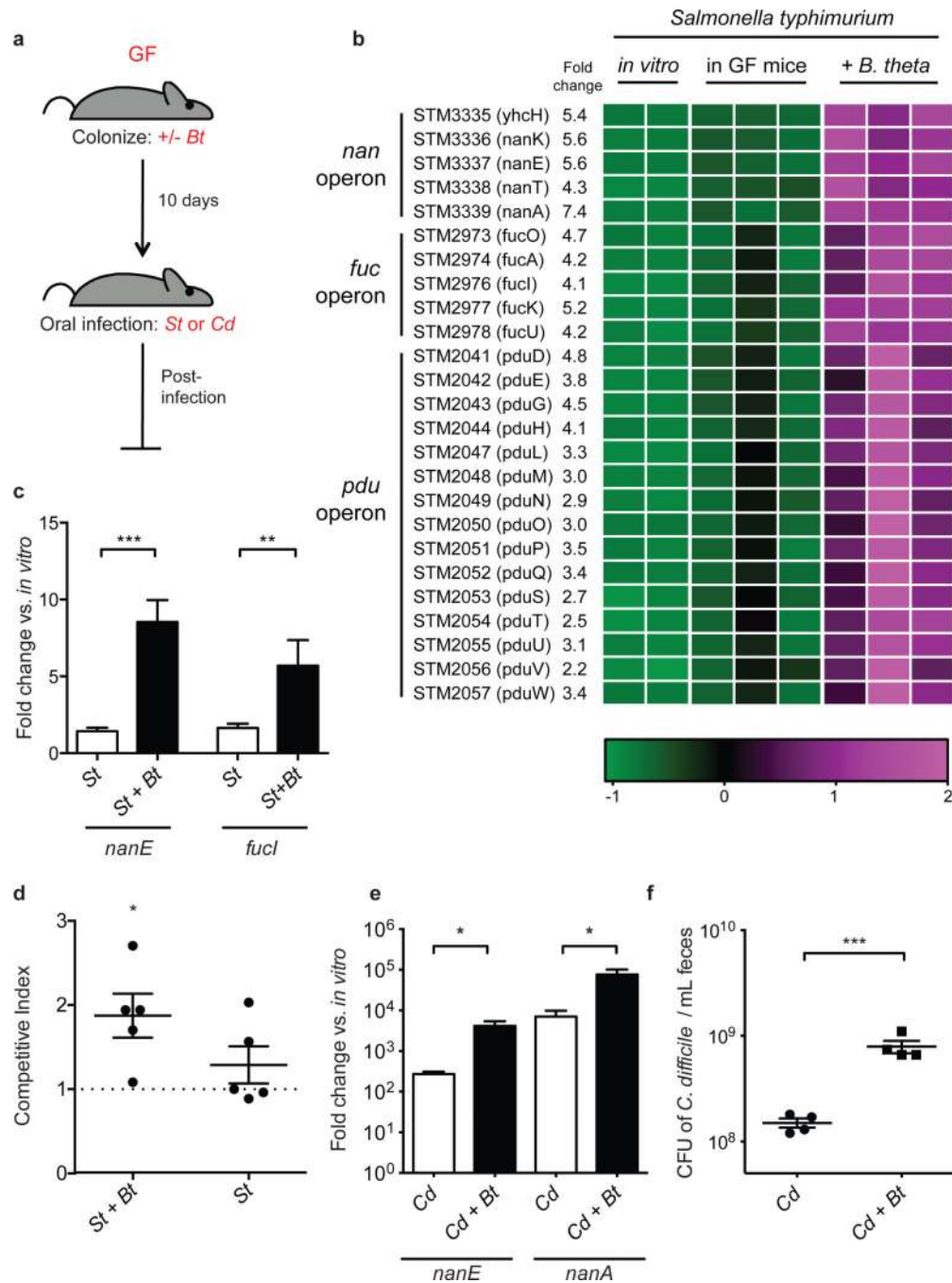
Figure 1. Bt facilitates S. typhimurium and C. difficile carbohydrate utilization during emergence a. Schematic of mouse infection experiments. Germ-free, GF; B. theta /iotaomicron, Bt; S. typhimurium , St; C. difficile , Cd.
