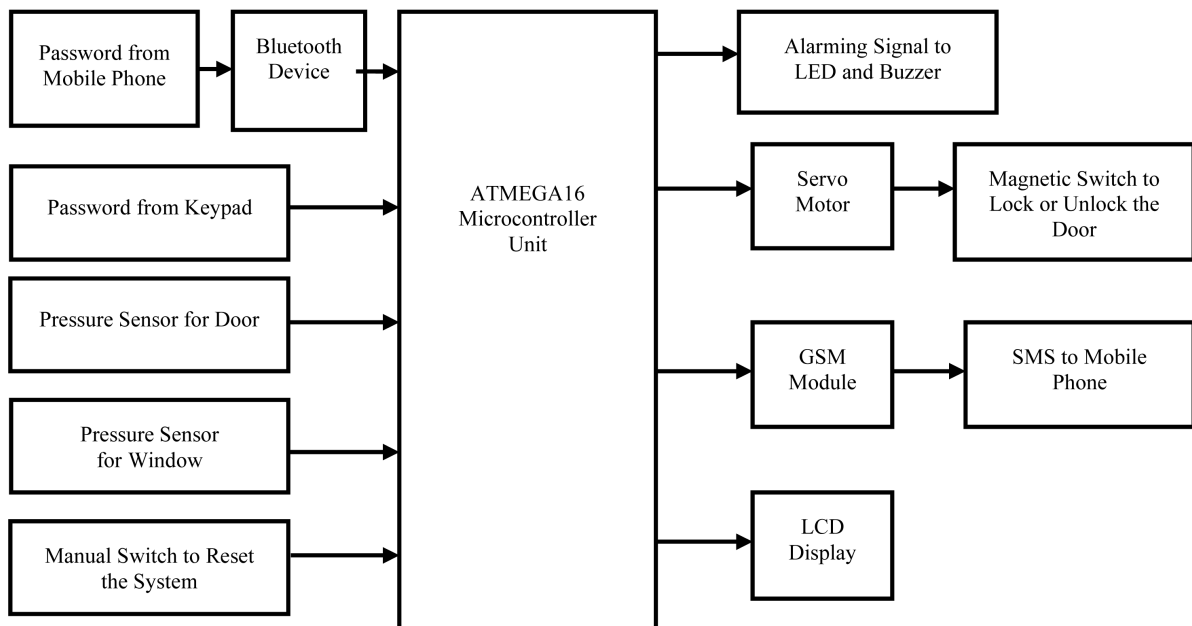
Figure 1. General block diagram of proposed home security system.
