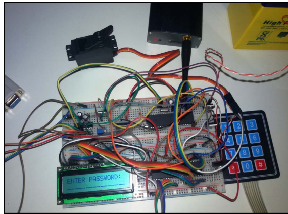
Figure 4. Hardware setup for home security system.
