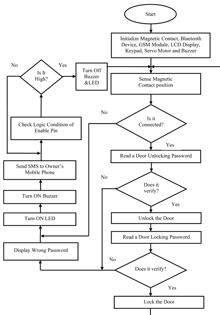
Figure 2. Program flow chart of the proposed home security system.
