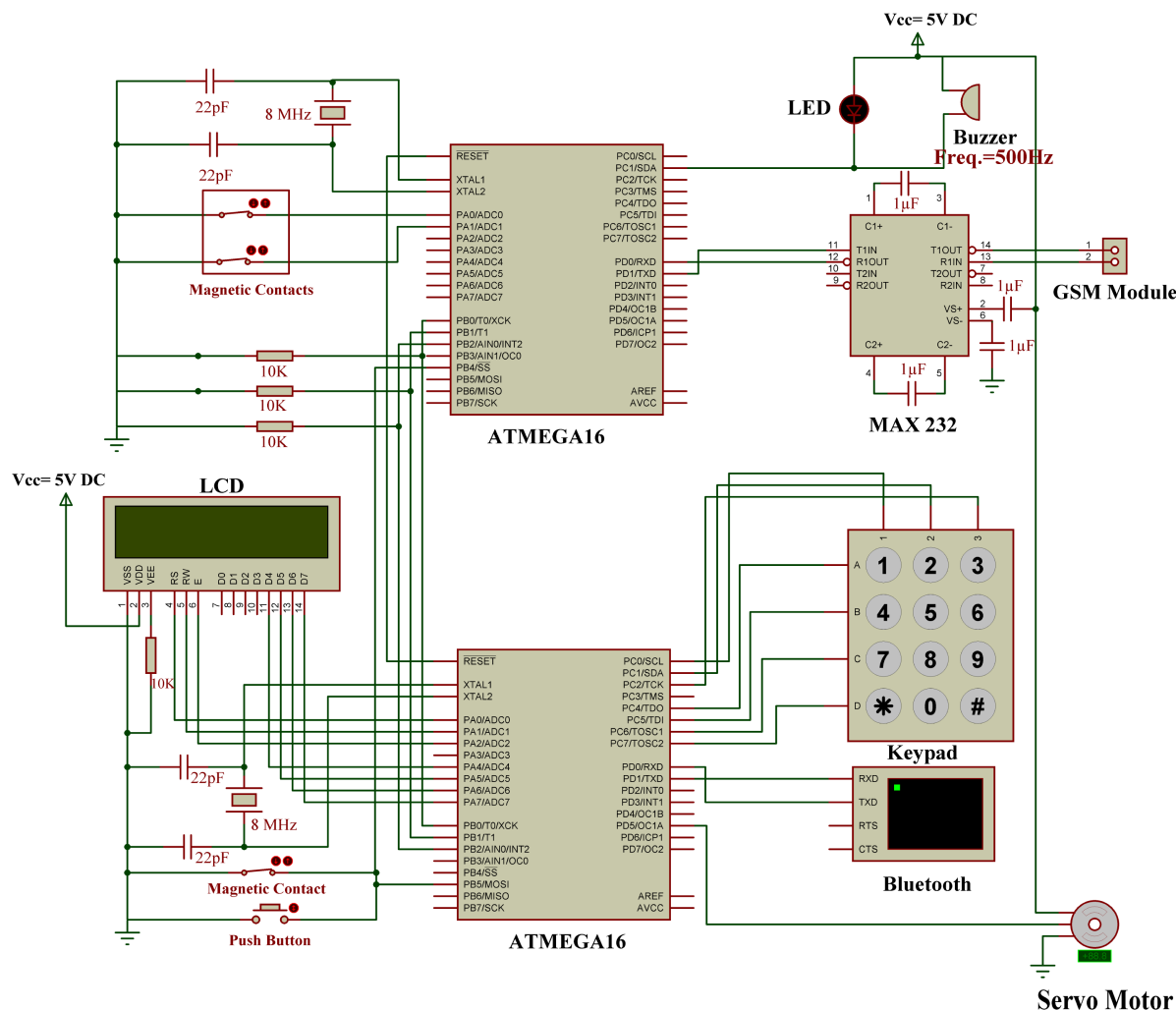
Figure 3. Schematic diagram of the proposed home security system.
