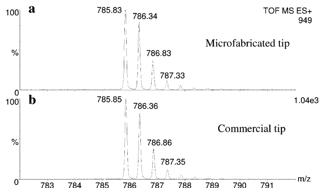
Figure 3. Mass spectra of 1 \mu\text{M} GFP B obtained from (a) a single-nozzle emitter ( 10 \mu\text{m} \times 8 \mu\text{m} ) and (b) a commercial capillary tip (i.d. \sim 10 \mu\text{m} ). Voltages of 4.5 and 2.1 kV were applied to the fabricated emitters and the commercial tips, respectively. The flow rate was 0.6 \mu\text{L}/\text{min} for all tips.
