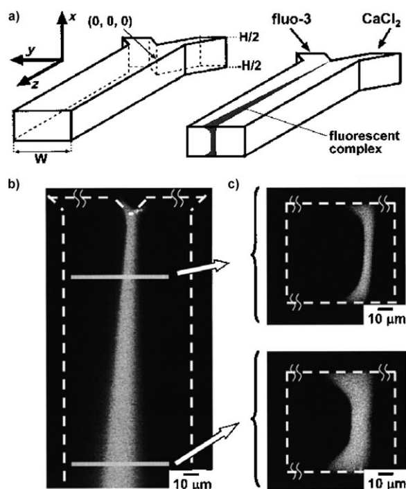
Figure 3. Images taken with a confocal microscope reveal significant deviations from the expected square root dependence. Due to the no-slip boundary condition, molecules near the walls spread with z^{1/3} rather than z^{1/2} (taken from ref. [17]).
