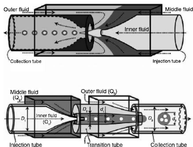
Figure 6. Top: Fabrication of a double emulsion in a co-flowing and flow-focusing device (taken from ref. [25]). Bottom: A device with two subsequent co-flowing streams in glass capillaries (taken from ref. [26]).
