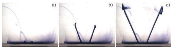
Figure 14. Fluid jets caused by an IDT at the bottom of a well covered by a small amount of dye. The fluid is contained in a cuvette, the part shown in the pictures is approximately 18 mm wide. Between the snapshots time spans of 0.16 s and 0.48 s have elapsed.
