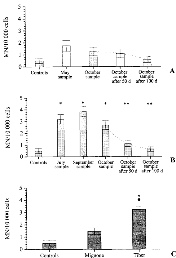
Fig. 3. Mean micronucleus frequencies (MN/10000 erythrocytes) in: (A) wild barbels from the Mignone river (May and October 1993 samples); (B) wild barbels from the Tiber river (July, September and October 1993 samples). In both cases barbels of the October sample were tested for MN at capture, after 50 and 100 days of maintenance in tanks. A total of 10000 erythrocytes per individual were analyzed; and (C) wild barbels from the Mignone river (samples from all seasons pooled) and in wild barbels from the Tiber river (samples from all seasons pooled). Controls are fish obtained by artificial reproduction and maintained in controlled conditions * Micronucleus frequency significantly higher ( p < 0.01 ) than the control value, using the Mann–Whitney U -test. ** Micronucleus frequency significantly lower ( p < 0.01 ) than the value at capture, using the Mann–Whitney U test. * Micronucleus frequency significantly higher ( p < 0.01 ) than the Mignone value, using the Mann–Whitney U test.
