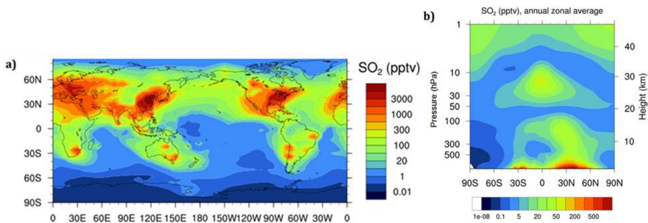
Fig. 3. (a) Calculated surface SO 2 mixing ratio; annual average as a function of latitude and longitude. (b) Calculated SO 2 mixing ratio; annual and zonal average as a function of atmospheric pressure and latitude.
