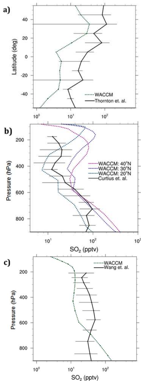
Fig. 4. (a) Calculated SO 2 concentration between 8–12 km at varying latitudes compared to an average of Pacific Exploratory Mission (PEM)-West A, PEM-West B, and Atmospheric Chemistry Experiment (ACE)-2 aircraft observations over the Pacific Ocean between 110° E and 80° W, binned into 10-degree segments with error bars representing plus/minus one standard deviation (Thornton et al., 1999). Model calculations are an annual average in the same longitude and altitude region. (b) Vertical profiles of calculated SO 2 mixing ratio at different latitudes compared to ACE-2 aircraft observations (Curtius et al., 2001). Observations are an average and standard deviation of 6 flights in July 1997 from 28° N to 32° N. Simulation lines are an average of the month of July at each of the latitudes noted. (c) Vertical profile of calculated SO 2 mixing ratio between 30° N and 30° S compared to PEM-TB aircraft observations (Wang et al., 2001). Observations are an average and standard deviation of DC-8 flights between 38° N and 36° S in March and April 1999. Simulation is an average of March and April from 38° N to 36° S.
