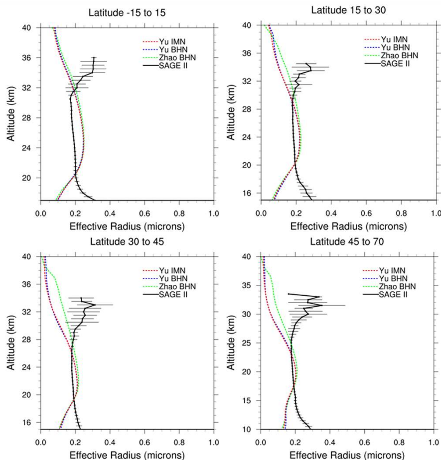
Fig. 8. Calculated sulfate effective radius compared to SAGE II satellite retrievals at the latitude regions specified. SAGE data are averaged from years 2000–2005. Simulations are 1-year average, using wet particle radii for calculations.
