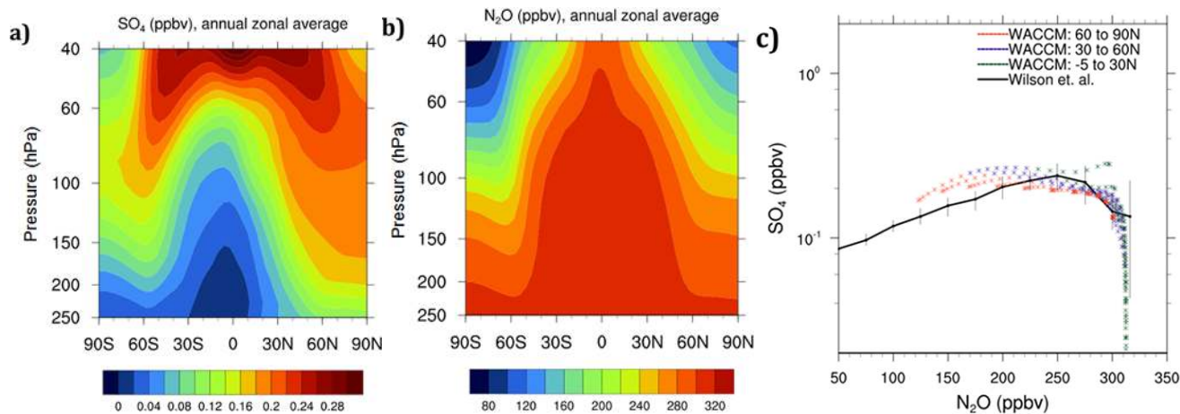
Fig. 6. (a) Calculated \text{SO}_4 mixing ratio; annual and zonal average as a function of atmospheric pressure and latitude. (b) Calculated \text{N}_2\text{O} mixing ratio; annual and zonal average as a function of atmospheric pressure and latitude. (c) Calculated \text{SO}_4 mixing ratio versus \text{N}_2\text{O} compared to a compilation of aircraft observations (Wilson et al., 2008). Observations are an average of volcanically quiescent aircraft observations between 1999 and 2004 taken from NASA ER-2, WB-57 and DC-8. The aircraft measurements spanned 5^\circ\text{S} to 90^\circ\text{N} latitude and approximately 40 to 250 hPa. Simulation points are annual zonal average of each grid cell between 40 and 250 hPa at the latitudes specified.
