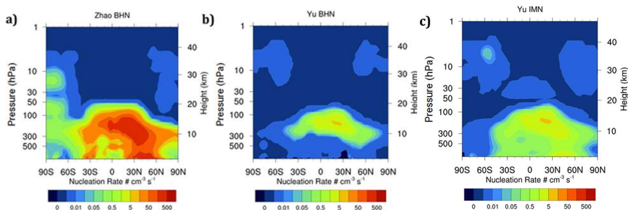
Fig. 12. Calculated nucleation rates; annual and zonal average as a function of atmospheric pressure and latitude. (a) Zhao BHN. (b) Yu BHN. (c) Yu IMN.
