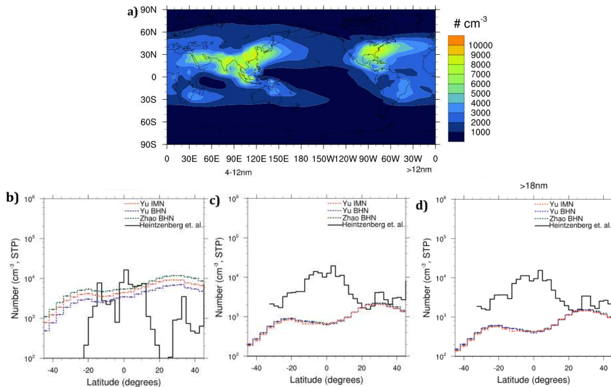
Fig. 15. (a) Calculated number concentration greater than 4 nm dry diameter as a function of latitude and longitude, using an annual average of the Zhao BHN simulation between 216–316 hPa (approximately 8.5–11.3 km). Comparison of zonal-average number concentrations to aircraft observations as a function of latitude over the altitude region 8.5–11.3 km for three particle diameter ranges: (b) 4–12 nm, (c) >12 nm, and (d) >18 nm. Observations are averages of 6 commercial flights between Germany, Namibia, and South Africa in May, July, and December 2000 (Heintzenberg et al., 2003). Simulations are annual and zonal averages at the bin ranges closest to the dry diameters specified (4.0 nm, 12.8 nm, and 16.2 nm diameters, respectively).
