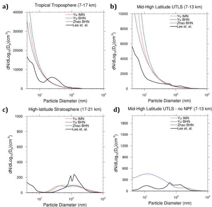
Fig. 13. Size distributions, corrected for STP, for the 3 calculated nucleation schemes compared to observed size distributions from 56 NASA flights between 1998–2000 as reported by Lee et al. (2003). Size distributions when recent NPF was observed at three different regions: (a) tropical troposphere, (b) mid-high latitude UTLS, and (c) high-latitude stratosphere. Observations define recent NPF when two conditions are met: (i) number concentrations with diameter 4–6 nm exceeding that of number concentration with diameter 6–9 nm, and (ii) number concentrations with diameter 4–9 nm exceeding 1 \text{ cm}^{-3} . Simulations were subjected to the same criteria by analyzing daily averages across the third simulation year for all grid boxes within the region. Simulation size bin ranges are selected based on the closest bins available to the size specified in Lee et al. (d) Size distributions in the mid-high latitude UTLS when recent NPF was not observed. Here, only the Yu BHN simulation is plotted because the Zhao BHN and Yu IMN schemes did not predict any days with no NPF.
