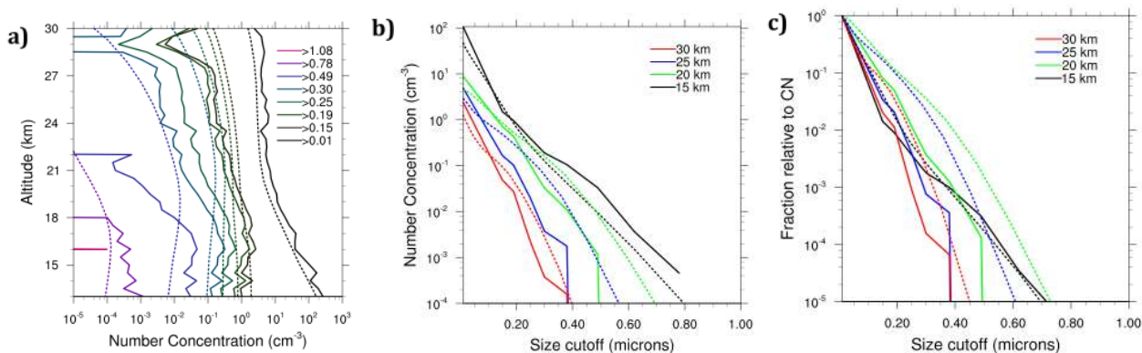
Fig. 9. Calculated size distributions for the Zhao BHN simulation (dotted lines) compared to balloon-borne observations above Wyoming (Deshler et al., 2003) (solid lines) at specified wet particle radii in microns. Observations are an average of years 2000–2010. Simulations are an annual average at 41^{\circ} N and 104^{\circ} W. (a) Vertical profile of number concentration larger than specified minimum radii. Calculated number concentrations were calculated using the closest bin to the specified wet radius. (b) Number concentration larger than a specified wet radius cutoff at the altitudes specified. (c) Ratio of number concentrations larger than the specified wet radius to number concentrations of condensation nuclei ( >0.01 microns wet radius).
