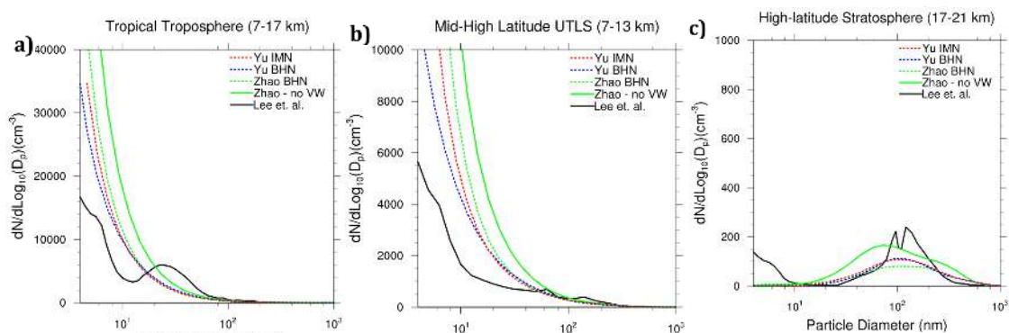
Fig. 14. Same as Fig. 13 except all simulation grid boxes are averaged, regardless of whether they met the criteria for recent NPF.
