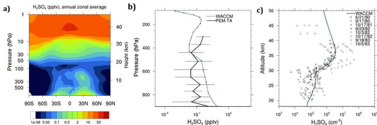
Fig. 5. (a) Calculated \text{H}_2\text{SO}_4 mixing ratio; annual and zonal average as a function of atmospheric pressure and latitude. (b) Vertical profile of calculated \text{H}_2\text{SO}_4 mixing ratio compared to PEM-TA (Bates et al., 1998; Hoell et al., 1999) aircraft observations binned into averages plus/minus standard deviation at different altitudes (Lucas and Prinn, 2003) from flights in August and September 1996 between 24^\circ\text{N} and 24^\circ\text{S} . Simulation lines are an average of July and August between 24^\circ\text{N} and 24^\circ\text{S} . (c) Vertical profile of calculated \text{H}_2\text{SO}_4 number concentration at 43^\circ\text{N} compared to various balloon-borne observations at the same latitude (Arnold et al., 1981; Reiner and Arnold, 1997; Schlager and Arnold, 1987; Viggiano and Arnold, 1981). Simulation is an average of the months of September and October while the observations were taken at the dates listed.
