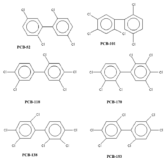
Fig. 2 Chemical structures of common PCB congeners found on microplastic surface from beaches
