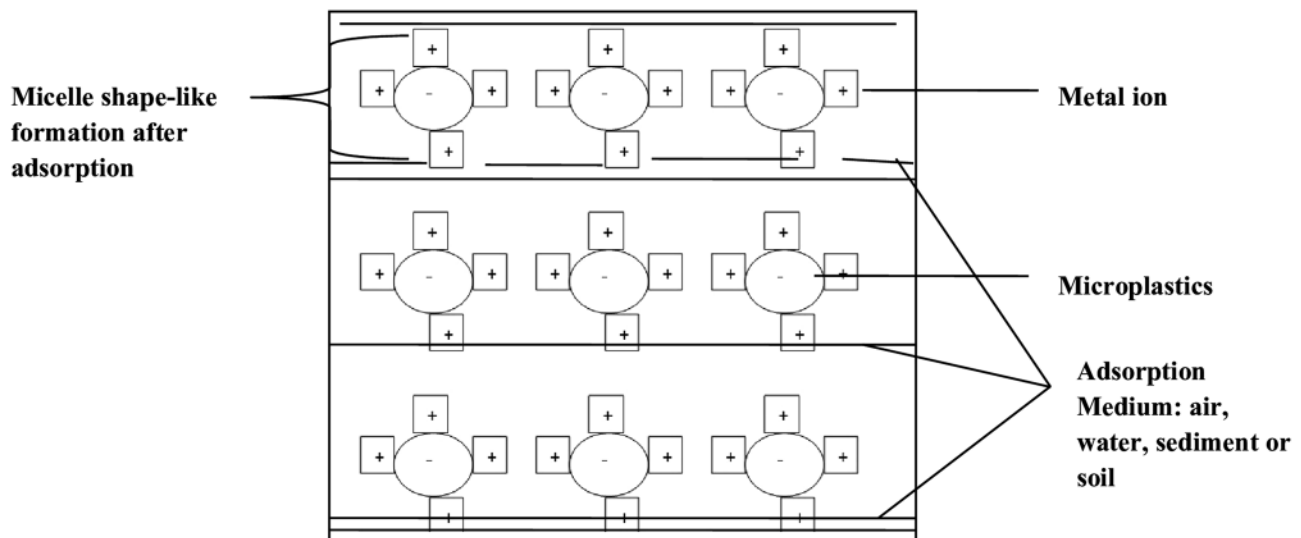
Fig. 4 Schematic of adsorption of metal ion onto microplastic
