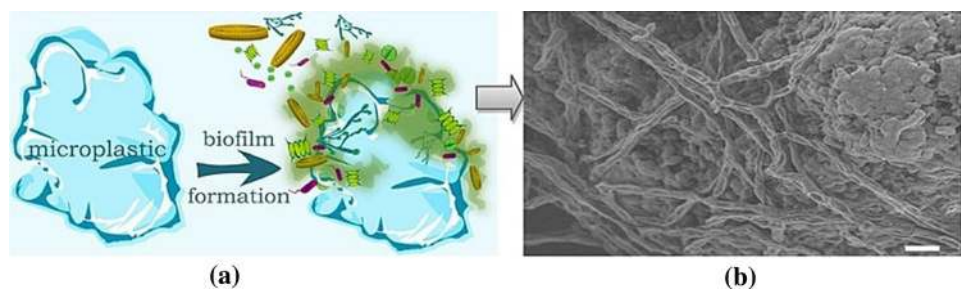
Fig. 5 a Biofilm formation on the surface of microplastic [19]. b Scanning electron micrograph showing a biofilm attached to a microplastic [63]
