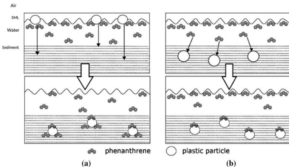
Fig. 3 Mechanisms of transfer of contaminants when: a Clean microplastics are presented in SML, and b clean microplastics are presented in sediment
