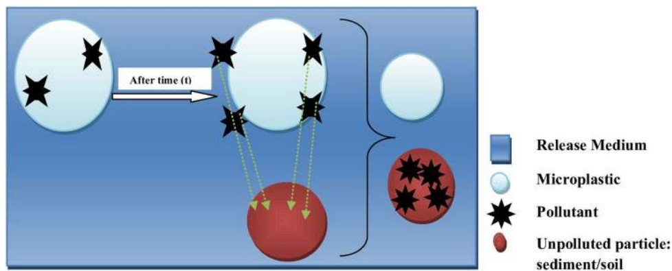
Figure 7 Graphical illustration of possible desorption/release mechanism of pollutants from microplastic surface onto clean/unpolluted particle. The adsorbed pollutant (black star) on the basis of concentration gradient, release distance and biofilm
