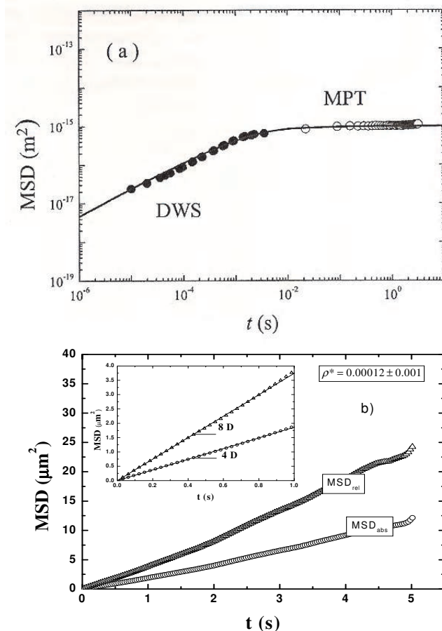
Fig. 4. a) Typical results of mean square displacement for a 3D gel made out of a polysaccharide in water [44]. Filled points are from DWS experiments, and open symbols are from particle tracking. The continuous line is an eye guide. b) Mean square displacement ( \text{MSD}_{\text{abs}} ), circles, and relative square displacement ( \text{MSD}_{\text{rel}} ), triangles, for latex particles at the water/n-octane interface. Experimental details: set of 300 latex particles of 1 \mu\text{m} of diameter, surface charge density: -5.8 \text{ mC cm}^{-2} , and reduced surface density, \rho^*=1.2 \cdot 10^{-3} ( \rho^*=\rho a^2 ), 25 ^\circ\text{C} . Figure 4.a is reproduced from Vincent et al. (2007). Inset corresponds to a smaller time interval.
