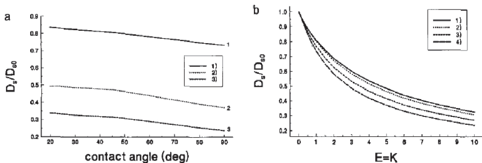
Fig. 7. Left: Effect of contact angle on the diffusion coefficient of a particle trapped at a fluid interface according to Danov's theory. D_{s0} is the diffusion coefficient for the bare interface. The different lines correspond to the following values of E (=K) : 1) 0; 2) 1; 3) 5. Right: Effect of the surface to bulk shear viscosity on the diffusion coefficient. The different lines correspond to the following values of E (=K) : 1) 0; 2) 1; 3) 5; 4) 10. Figures reproduced from Dimova et al. (2000).
