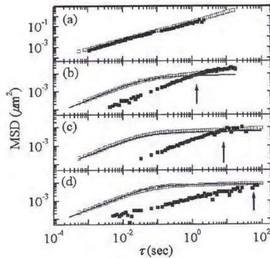
Fig. 5. Comparison of one-particle (open symbols) and two-particle (closed symbols) MSD for a solution of F-actin using particles of radius 0.42 \mu\text{m} . Different average actin filaments are used: a) 0.5 \mu\text{m} , b) 2 \mu\text{m} , c) 5 \mu\text{m} , d) 17 \mu\text{m} . Notice that when the scale of the inhomogeneities of the solution is similar to the particle size both methods lead to the same results. The figure is reproduced from Liu et al. (2006).
