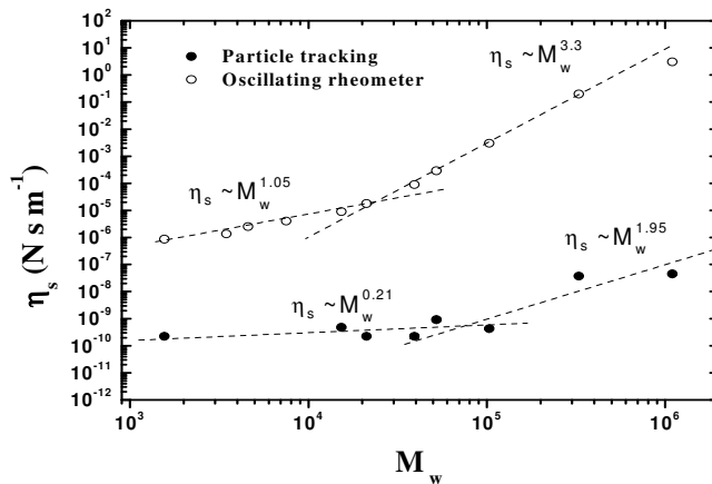
Fig. 10. Surface shear viscosity for monolayers of poly(t-butyl acrylate) as a function of the molecular weight and for a surface pressure of 16 \text{ mN m}^{-1} . The lower curve corresponds to data obtained from particle tracking. The upper curve was obtained from conventional oscillatory rheometers.
