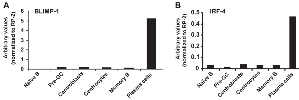
Fig. 4. Expression pattern of BLIMP-1 and IRF-4 transcription factors in plasma cells derived from human tonsils. (A) BLIMP-1, a transcription factor predicted to be bound by miR-125b is expressed only by plasma cells as determined by real-time PCR analysis. (B) IRF-4, a transcription factor predicted to be bound by miR-125b is expressed only by plasma cells as determined by real-time PCR analysis. Three independent tonsils were examined and a representative plot is shown. Values represent arbitrary numbers derived from Ct values normalized to RP-2 house keeping control.
