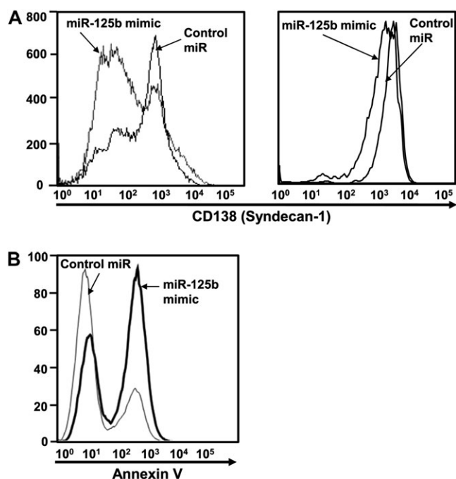
Fig. 6. Effects of miR-125b over-expression in a myeloma cell line. (A) CD138 expression in U266 myeloma cells transfected with control mimic or miR-125b mimic (left panel) and CD138 expression in U266 myeloma cells infected with control virus or miR-125b-expressing lentivirus (right panel); (B) annexin V staining of myeloma cells transfected with control mimic or miR-125b mimic. Cells were stained for propidium iodide (PI) and annexin V. Annexin V + PI - cells are plotted as a histogram.
