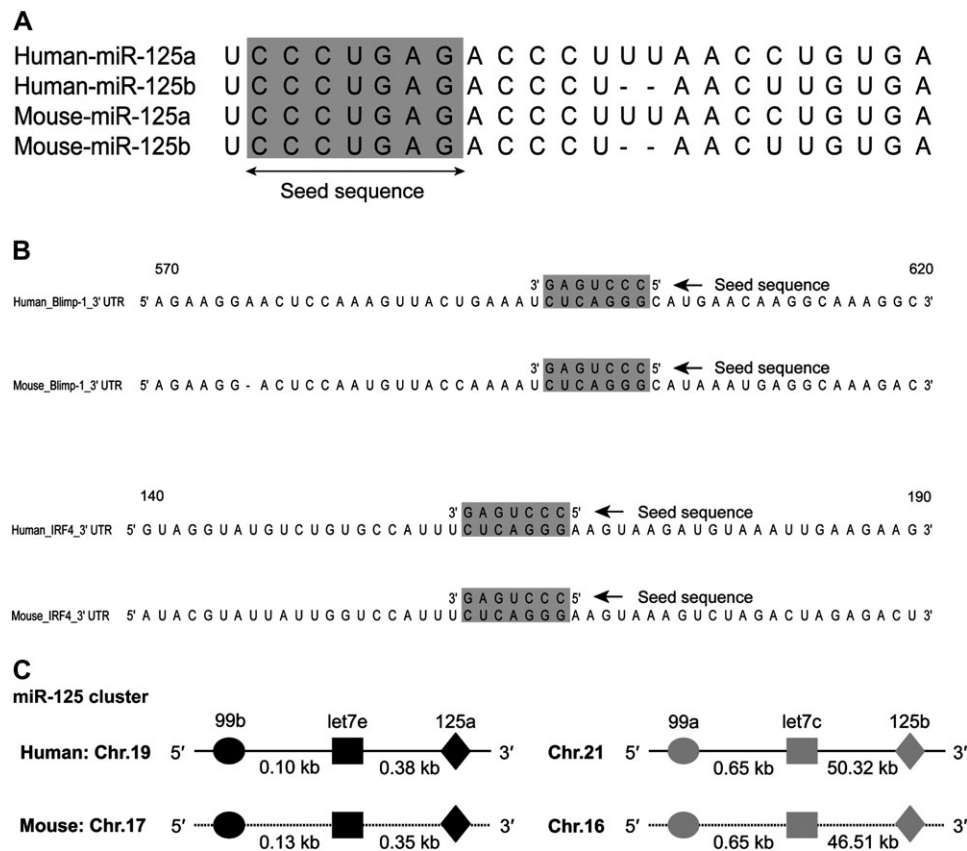
Fig. 1. Cluster analysis of miR-125 genes in mouse and human genomes. (A) Sequence conservation of miR125a and miR-125b in mice and humans. Alignment of mature miR125a and miR-125b sequences from human and mouse, respectively, is shown. The potential seed sequences are highlighted. (B) The predicted miR125 seed pairing with the 3' UTRs of BLIMP-1 and IRF-4 transcription factors. The positions in the alignment are based on the human BLIMP-1 and IRF-4 sequences. (C) Genomic organization of miR-125 clusters. The homologous relationships of miR-125b gene clusters are shown for human and mouse with the paralogous miRNA relationship represented by solid and grey shades. The physical distances between miRNAs in the chromosome (Chr) clusters are indicated. The figure is not drawn to scale.
