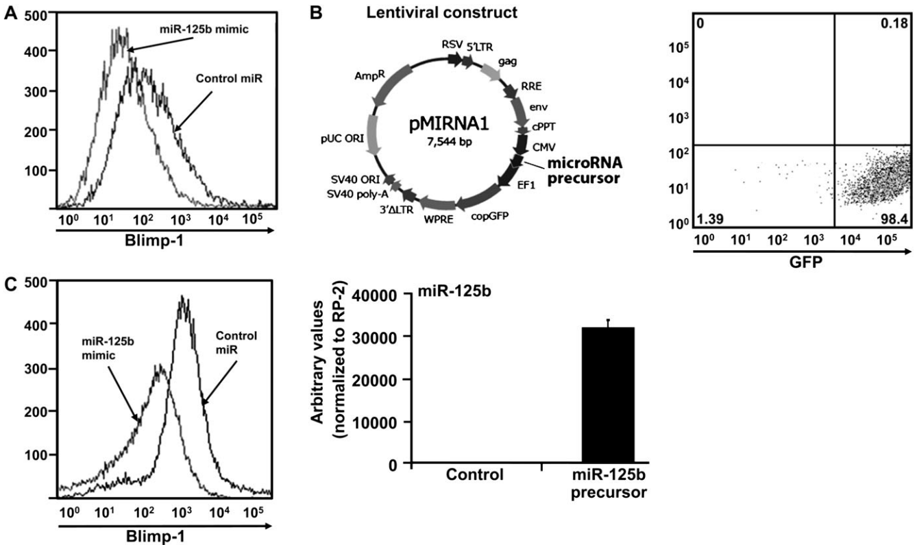
Fig. 5. BLIMP-1 protein levels in B cell lines over-expressing miR-125b. (A) Flow cytometric analysis of intracellular BLIMP-1 expression in Bcl1.3B3 mouse cells infected with control virus or miR-125b-expressing virus treated with 20 \mu\text{g ml}^{-1} of LPS. (B) miR-125b precursor mimic cloned into a lentiviral vector that co-expresses GFP or the control vector were transduced into U266 myeloma cell line (top left panel). GFP + cells were sorted 72 h after infection and cultured in vitro (top right panel). Detection of lentivirus-mediated miR-125b expression in U266 cells by real-time PCR (bottom left panel). (C) Flow cytometric analysis of intracellular BLIMP-1 expression in U266 myeloma cells infected with control virus or miR-125b-expressing virus.
