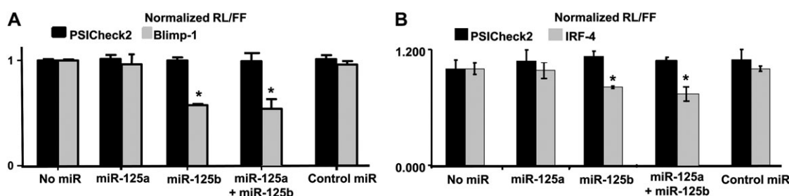
Fig. 3. miR-125b but not miR-125a binds to 3' UTR of BLIMP-1 and IRF-4 mRNAs. Dual luciferase activity of reporter plasmids with the wild-type 3' UTR of BLIMP-1 (panel A) or IRF-4 (panel B) fused to the luciferase gene upon miR-125a or miR-125b precursor co-transfection of the same reporter vector with the non-targeting control. Results are expressed as relative luciferase (RL) units normalized to firefly luciferase (FF) units in triplicate analyses from two experiments. Statistical comparisons between the co-transfected miRNA and the non-targeting control for the same reporter vector were performed and P values < 0.05 are indicated by *. Bars correspond to the SEM. Statistical comparisons were performed by 2-tailed t -test.
