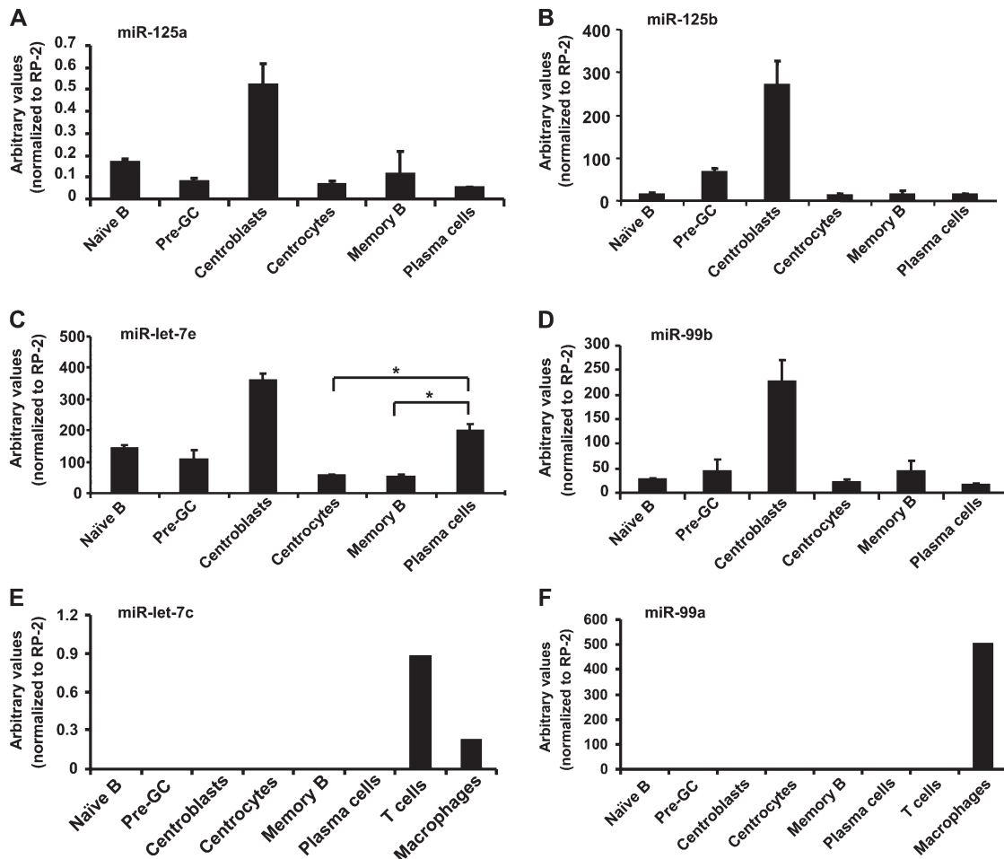
Fig. 2. Expression profiling of miR-125 genes in human B cells. Real-time PCR analysis indicates that miR-125a (A), miR-125b (B), miR-let-7e (C) and miR-99b (D) are preferentially expressed by centroblasts in the GC. miR-let-7c (E) and miR-99a (F) are expressed by T cells and macrophages, respectively. Three independent tonsils were examined and a representative plot is shown. Values represent arbitrary numbers derived from Ct values normalized to RP-2 house keeping control. Statistical analysis of miRNA expression was done by the Student's t -test and P value <0.05 are indicated by asterisks. Bars indicate SEM.
