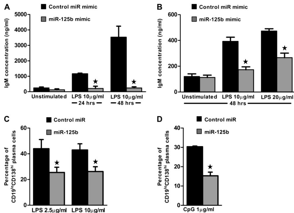
Fig. 7. miR-125b effects on the induction of plasma cell differentiation and antibody secretion. (A) Bcl1.3B3 murine B cell line was co-transfected at a 2:1 ratio of either control miRNA mimic or miR-125b mimic and a GFP plasmid. GFP + cells were sorted by flow cytometry-based cell sorter and cells were treated with toll-like receptor agonist LPS ( 10 \mu\text{g ml}^{-1} ) that induces differentiation of this cell line. Supernatants were harvested 48 h post-LPS stimulation and IgM was quantified by ELISA. Statistical analysis of IgM quantification was done by the Student's t -test and P < 0.05 was considered significant comparing control miR mimic and miR-125b mimic in the presence of LPS. This experiment was repeated twice and a representative experiment is shown. (B) Lentiviral-mediated stable expression of miR-125b precursor mimic in Bcl1.3B3 mouse cells and cultured in the presence or absence of LPS. Supernatants were harvested 48 h post-LPS stimulation and IgM was quantified by ELISA. Statistical analysis of IgM quantification was done by the Student's t -test and P < 0.05 was considered significant comparing control virus-expressing cells and miR-125b mimic-expressing cells in the presence of LPS. (C) Retroviral-mediated expression of miR-125b precursor mimic in splenic B cells cultured in the presence or absence of different doses of LPS. Cells were harvested on day 6 and analyzed for CD19 and CD138 expression by FACS analysis of GFP + cells. This experiment was repeated four times and the plot derived from all these experiments is shown. Significant differences between control miR and 125b miR in four experiments showed P values < 0.05 and correspond to the SEM. (D) Retroviral-mediated expression of miR-125b precursor mimic in splenic B cells cultured in the presence or absence of 1 \mu\text{g ml}^{-1} of CpG. Cells were harvested on day 6 and analyzed for CD19 and CD138 expression by FACS analysis of GFP + cells. This experiment was repeated thrice and the plot derived from these experiments is shown. Differences between control miR and 125b miR in three experiments showed P values < 0.05 and bars correspond to the SEM.
