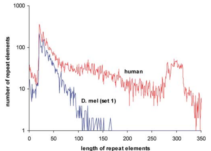
Figure 7. Length Distribution of Repeat Elements in 3' UTRs of Human and D. melanogaster
