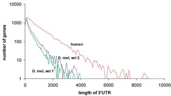
Figure 6. Lengths Distribution of 3' UTRs in Human and D. melanogaster Data for set 1 and set 2 on a logarithmic scale. The distribution decays exponentially with increasing length in human much slower than in D. melanogaster . The average 3' UTR lengths in human and D. melanogaster are approximately 900 and approximately 400 nucleotides, respectively. DOI: 10.1371/journal.pcbi.0010013.g006
