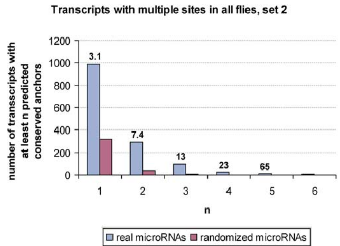
Figure 4. Specificity of PicTar Predictions of Genes with Multiple Putative Target Sites Number of unique genes as a function of the minimal number of anchor sites for 46 unique, conserved microRNAs and for randomized microRNAs (averaged over five cohorts). The ratio of these numbers, reflecting the specificity, is indicated above each bar. DOI: 10.1371/journal.pcbi.0010013.g004
