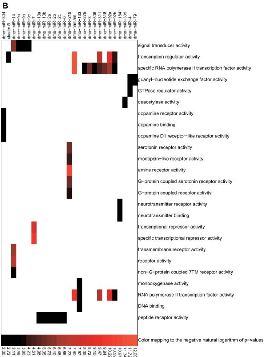
Figure 5. Significant GO Terms among the Predicted Target Genes of All Single microRNAs and Clusters of Co-Expressed microRNAs Significantly enriched GO terms for (A) “biological processes” and (B) “molecular function” ontologies. Shown are GO terms with p -values smaller than 0.1, corrected for multiple testing. Hierarchical clustering was performed separately for GO terms and microRNAs (see Materials and Methods). DOI: 10.1371/journal.pcbi.0010013.g005
