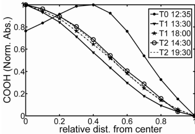
Figure 7. COOH radial scans inferred from STXM/NEXAFS analysis of particles having inorganic inclusions. At the urban site (T0), the inorganic inclusions were located at the center of the particle, resulting in a lower COOH content at that location of the particle. At T1 and T2, the inorganic material was typically not located at the center of the particles as indicated by the fact that the COOH absorption was highest there. Each line represents an average of 24 (at T1) to 121 (at T0) particles.
