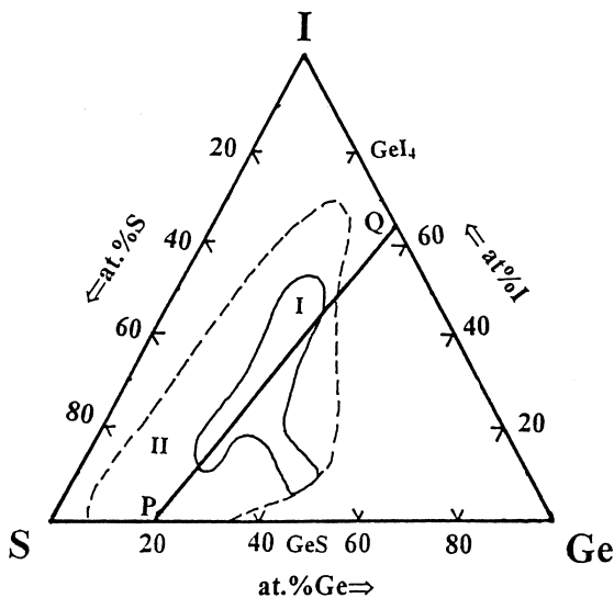
Fig. 1. Glass forming region in the Ge–S–I ternary taken from the work of Dembovsky et al. [9]. Glasses form in region II upon a water quench of melts. But of these only melt compositions in region I yield glasses when cooled very slowly at 2 \text{ K min}^{-1} , showing that the glass forming tendency is optimized in region I. Line PQ is the prediction of the glass forming tendency based on Eq. (3) from extended constraint theory.
