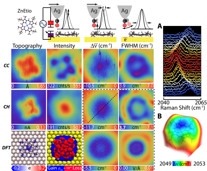
Fig. 2. ZnEtio on Au(111): Imaging principles of TERS-mfm are illustrated in the header. Simultaneously recorded STM topography and TERS-related images of intensity, frequency shift ( \Delta\nu ), and linewidth recorded under CC and CH scan mode. We low pass-filtered the intensity and linewidth maps for clarity. The \Delta\nu maps in CC and CH mode are referenced to 2058.6 and 2059.5 \text{ cm}^{-1} , respectively. The DFT results consist of the Löwdin projected atomic charges, deformation charge density, and vertical and lateral electric fields. (A) Stark tuning of the CO vibration along the dashed line in the CH \Delta\nu map. (B) Electrostatic field surface obtained by color-coding the Stark shift on the STM CH topography. The common image size is 23 \text{ \AA} \times 23 \text{ \AA} . The set point is 0.1 \text{ nA} , 1.2 \text{ V} .
