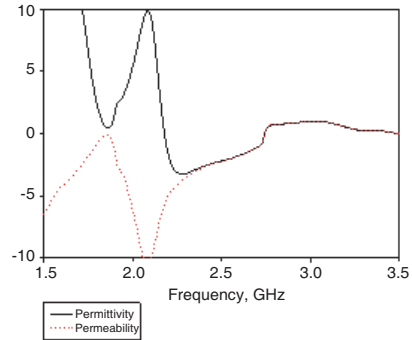
Figure 4. Value of \epsilon_r and \mu_r of the single cell LHM.
