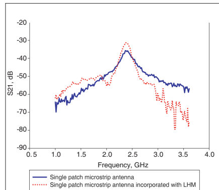
Figure 15. Gain ( S_{21} ) comparison between the single patch microstrip antenna with and without LHM.
