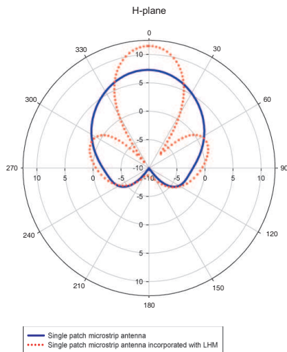
Figure 9. Simulated radiation pattern in H -plane.
