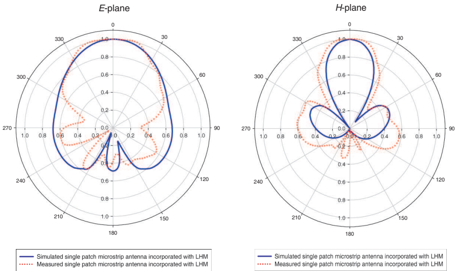
Figure 18. Comparison between simulated and measured radiation patterns in E -plane.
