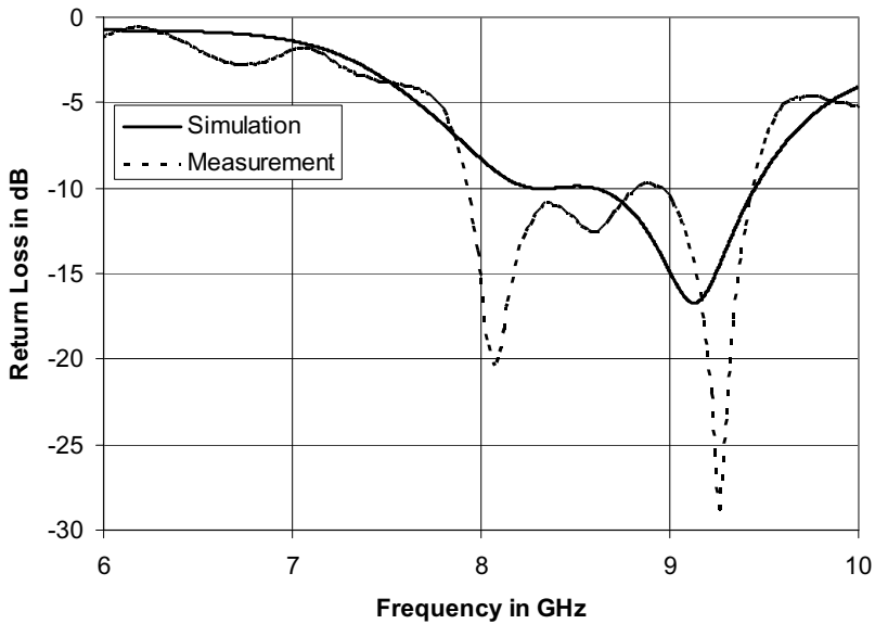
Figure 6. Computed and measured return loss vs. frequency for low profile DRA.
