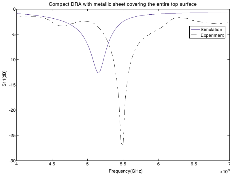
Figure 9. Computed and measured return loss vs. frequency for compact DRA with large metallic sheet.
