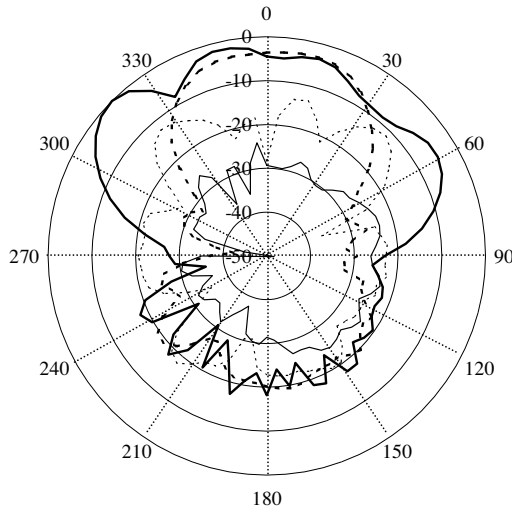
Figure 4. Measured radiation patten at 9 GHz (10 dB/Div) — E-Co, \dots\dots H-Co, — E-X, --- H-X.
