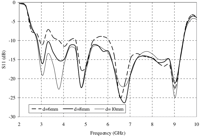
Figure 3. Measured return loss with different distances between the reflector and dielectric substrate ( d ) --- d = 6 mm, — d = 8 mm, —\diamond— d = 10 mm.
