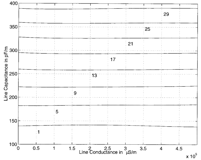
Fig. 5. Contour map of the real part of dielectric constant as a function of line conductance and capacitance for a microstrip line with \epsilon_s = 6.15 and w_s/h = 1.46 .
