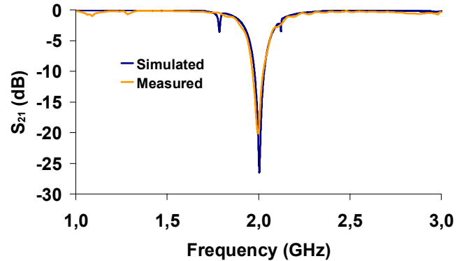
Fig. 6 Simulated and measured S_{21} (off state)
