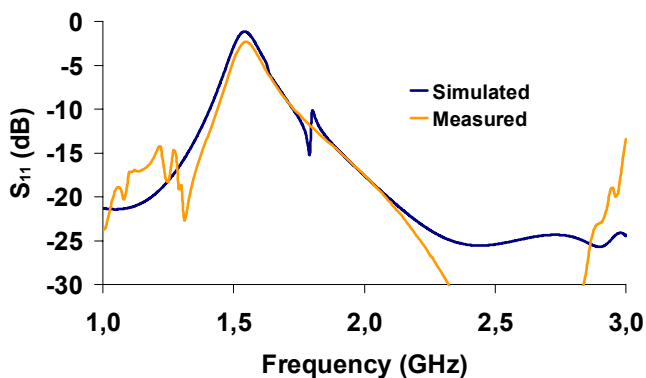
Fig. 9 Simulated and measured S_{11} (on state)
