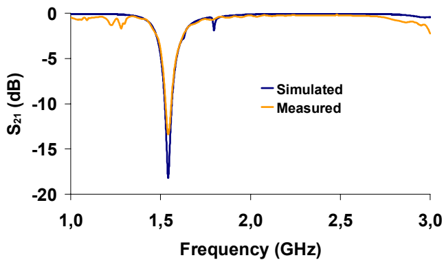
Fig. 8 Simulated and measured S_{21} (on state)
