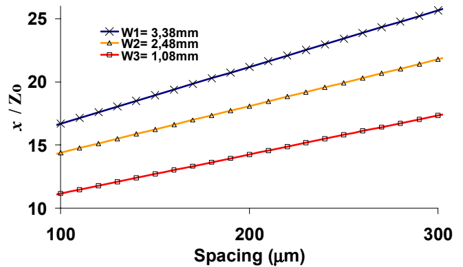
Fig. 2 Resonator spacing from the main transmission line vs normalized reactance slope parameter for different resonator widths
