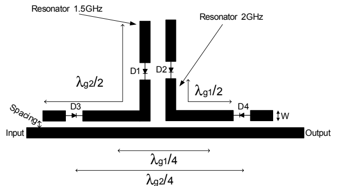
Fig. 3 Two-pole Switchable bandstop filter
