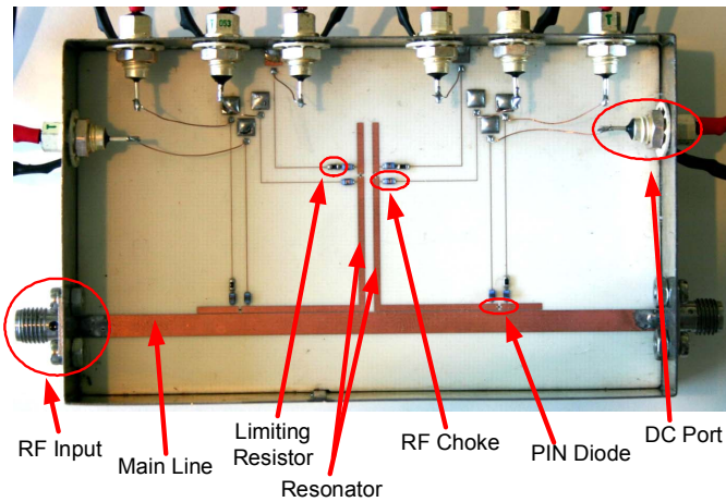
Fig. 5 Photograph of the switchable bandstop filter
