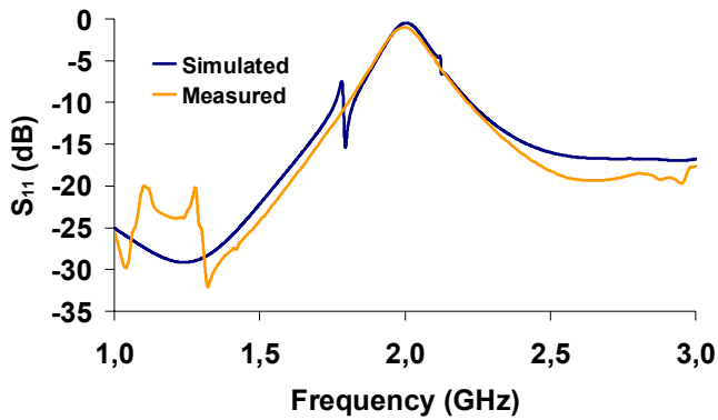
Fig. 7 Simulated and measured S_{11} (off state)
