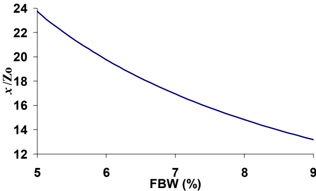
Fig. 1 Fractional bandwidth vs normalized reactance slope parameter of a single resonator coupled to the main line.
