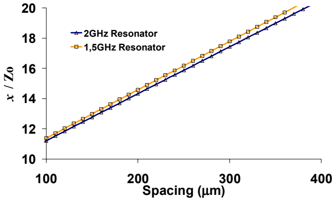
Fig. 4 Normalized reactance slope parameter vs resonator spacing from the main transmission line.
