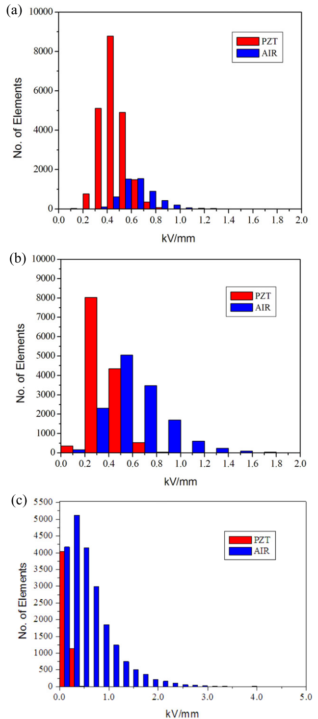
Figure 4. Electric field magnitude in through-thickness direction ( z ) for PZT and air cells at different PZT volume fractions (a) 80% PZT, (b) 50% PZT and (c) 20% PZT. Coercive field is 0.4 \text{ kV mm}^{-1} and applied field based on voltage/thickness is 0.5 \text{ kV mm}^{-1} .
