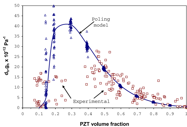
Figure 8. Variation of d_h \cdot g_h as a function of PZT volume fraction. Experimental data from [25, 26].
