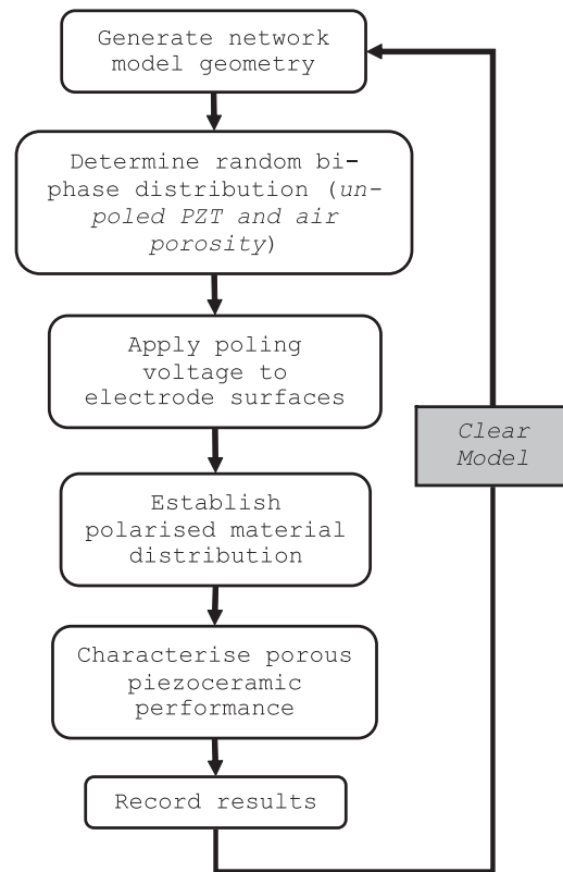
Figure 2. Flow chart showing the approach used to model porous piezoceramic structures, taking into account the initial unpoled state and simple polarization of the material.
