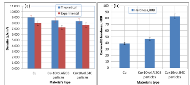
Fig. 2. Density (a) and hardness (b) of Cu matrix particle-reinforced composites.
