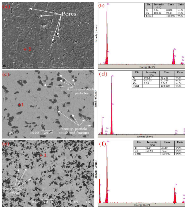
Fig. 1. Microstructure of the particle-reinforced composites. (a) Copper matrix, (b) EDS analysis of copper matrix, (c) \text{Al}_2\text{O}_3 particles, (d) EDS analysis of \text{Al}_2\text{O}_3 particles, (e) \text{B}_4\text{C} particles, (f) EDS analysis of \text{B}_4\text{C} particles.
