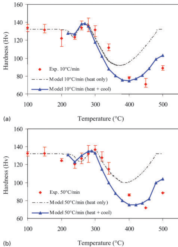
1 Model predictions of hardness of samples during non-isothermal heating at a 10 and b 50°C min -1 are compared with experimental results of hardness measured after heating at 10 and 50°C min -1 followed by cooling at 50°C min -1
