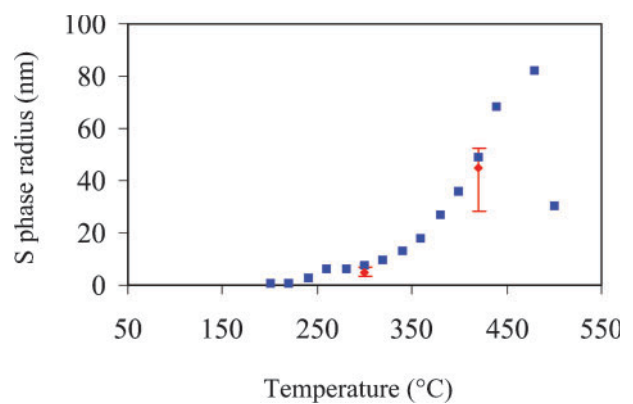
4 Model predictions of S phase radius during heating at 10°C min -1 are compared with average radius measured from TEM graphs after heating sample at 10°C min -1 up to 300 and 420°C followed by cooling at 50°C min -1
