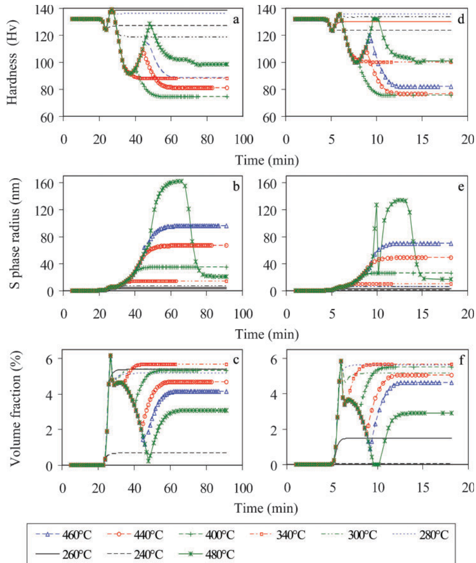
2 Model predictions of hardness, S phase average size and volume fraction as function of ageing time during non-isothermal heating at a-c 10 and d-f 50°C min -1 to peak temperature and followed by cooling to room temperature at 50°C min -1
