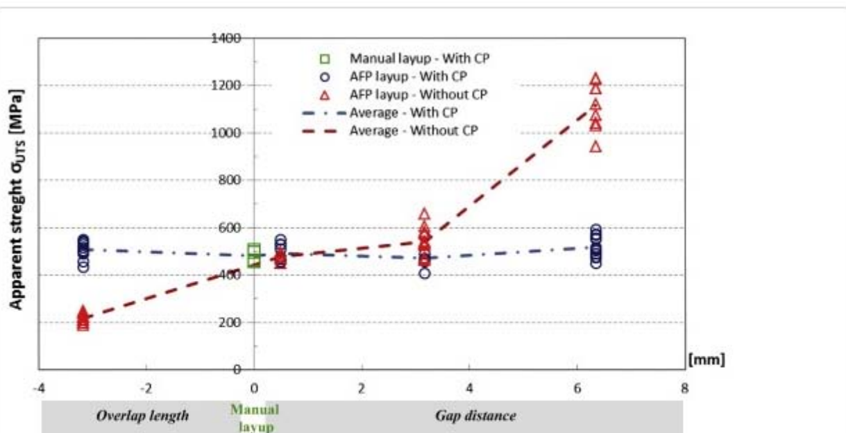
Fig. 11. Apparent tensile stress variation at failure as a function of the type of embedded defect with and without caul plate, [0^\circ/90^\circ_\varepsilon/0^\circ] . (For interpretation of the references to color in this figure legend, the reader is referred to the web version of this article.)
