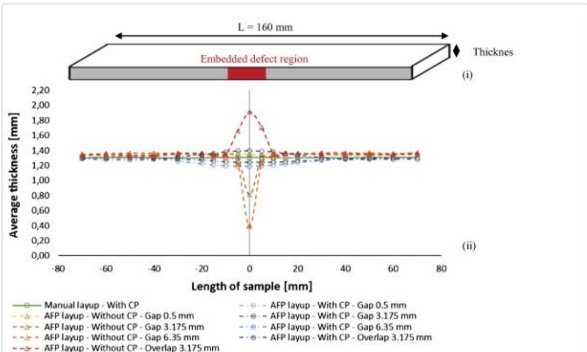
Fig. 6. (i) Specimen geometry for microstructure observations; (ii) Evolution of the thickness in the length of samples according to the embedded defects introduced during the draping phase, [0^\circ/90^\circ_\epsilon/0^\circ] . (For interpretation of the references to color in this figure legend, the reader is referred to the web version of this article.)
