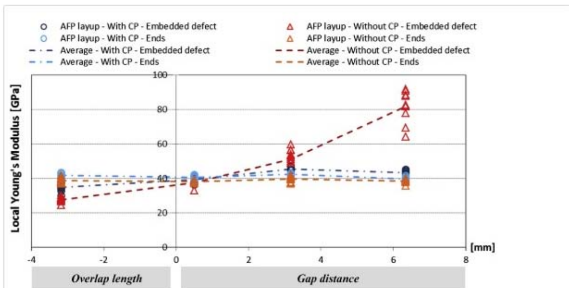
Fig. 9. Local elastic modulus variation (in the ends and embedded defect region of samples) as a function of the type of embedded defect with and without caul plate, [0^\circ/90^\circ_\pm/0^\circ] . (For interpretation of the references to color in this figure legend, the reader is referred to the web version of this article.)
