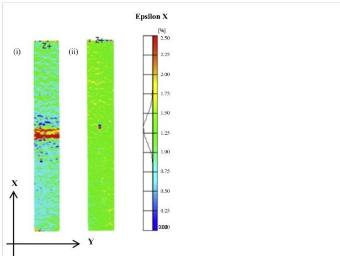
Fig. 8. Evolution of the axial deformation before rupture sample for gap 6.35 mm (ARAMIS): (i) Polymerized without caul plate; (ii) Polymerized with caul plate. (For interpretation of the references to color in this figure legend, the reader is referred to the web version of this article.)
