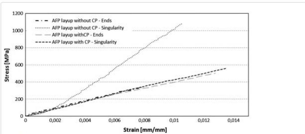
Fig. 7. Comparison of Stress-Strain for different gap 6.35 mm configuration (in the ends and embedded defect region of samples)
