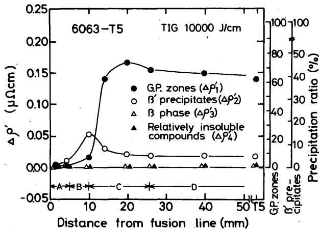
Fig. 9 Distribution of G.P. Zones ( \Delta\rho_1 ), \beta' precipitates ( \Delta\rho_2 ), \beta phase ( \Delta\rho_3 ) and relatively insoluble compounds ( \Delta\rho_4 ) in the HAZ of TIG welds of 6063-T5 alloy.
