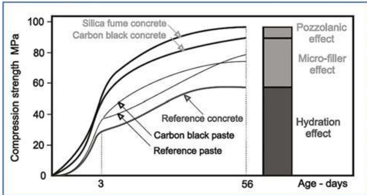
Figure 18. Hydration, pozzolanic, and filler effects of cementitious pastes with silica fume [28].
