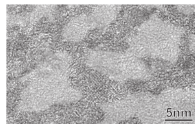
FIG. 2. Typical HREM image of Pd 42.5 Ni 7.5 Cu 30 P 20 metallic glass after annealing at 290 °C (below or near T_g ) for 10 h under ultrasonic vibrations of 0.35 MHz. The remaining amorphous fraction was estimated to be about 80% from the crystallization heat measured by differential scanning calorimetry. It can be clearly recognized that the amorphous domains are surrounded by crystallized walls that show lattice fringes. Ultrasonic vibrations are considered to accelerate crystallization of WBRs via \beta relaxation. The crystallized walls would be thin if annealing time is shortened. The sample for HREM was prepared by ion milling with cooling using liquid N 2 to prevent crystallization due to ion irradiation. For the sake of conspicuity of the boundaries, the amorphous-like regions are colored grey.
